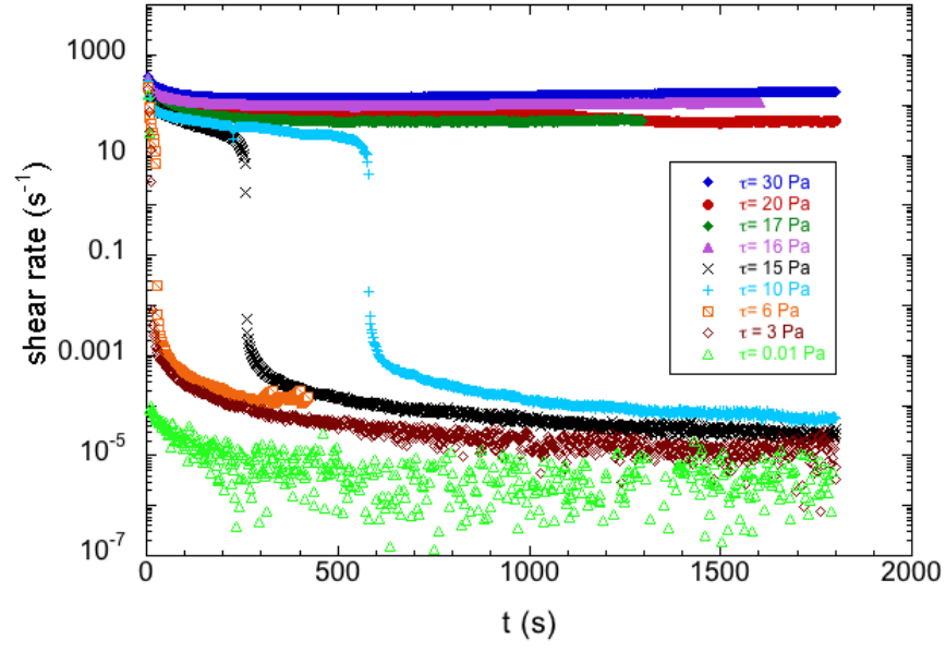
Figure 3: Creep tests for the 40% THF weight concentration, at T = 1^\circ\text{C} .
