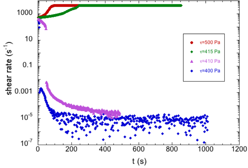
Figure 1: Creep test for the 30% THF weight concentration, at T = 1^\circ\text{C} .
