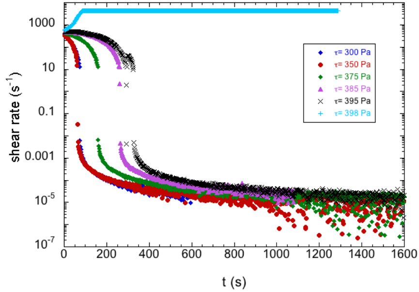
Figure 2: Creep tests for the 35% THF weight concentration, at T = 1^\circ\text{C} .
