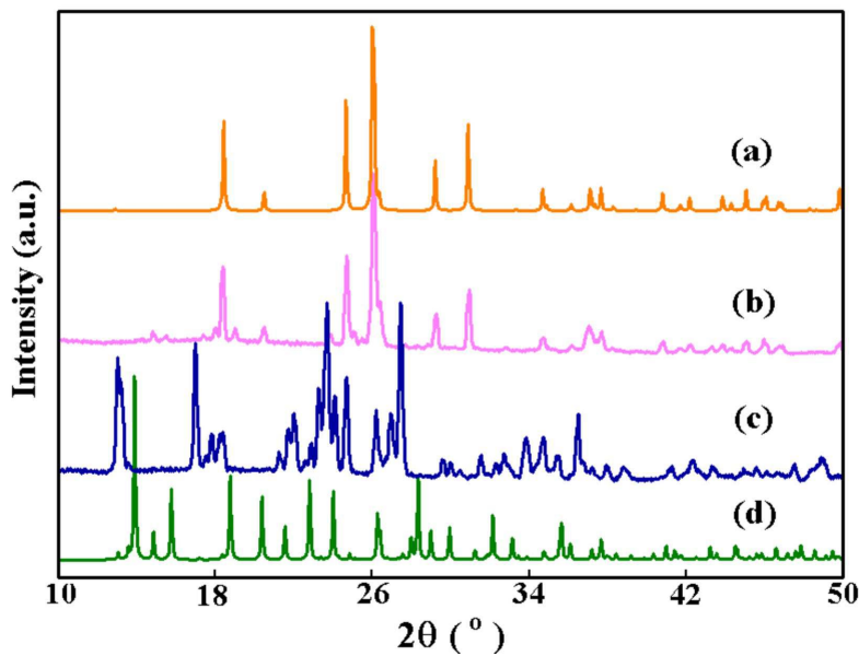
Figure S2. Powder X-ray diffraction patterns for (a) \text{CuReO}_4 (theoretical), (b) TGA residue after second weight loss step from I , (c) TGA residue after first weight loss step from I , and (d) freshly prepared \text{CuReO}_4(\text{pyz}) .
