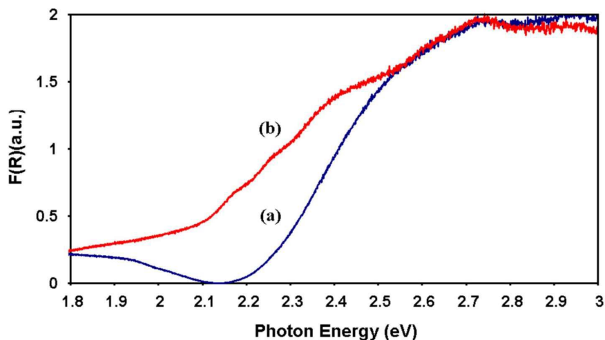
Figure S1. A plot of UV-vis diffuse reflectance spectra, F(R) vs. photon energy, (a) the residual of the first step TGA of II , (b) the residual \text{CuReO}_4 of the final TGA of II .
