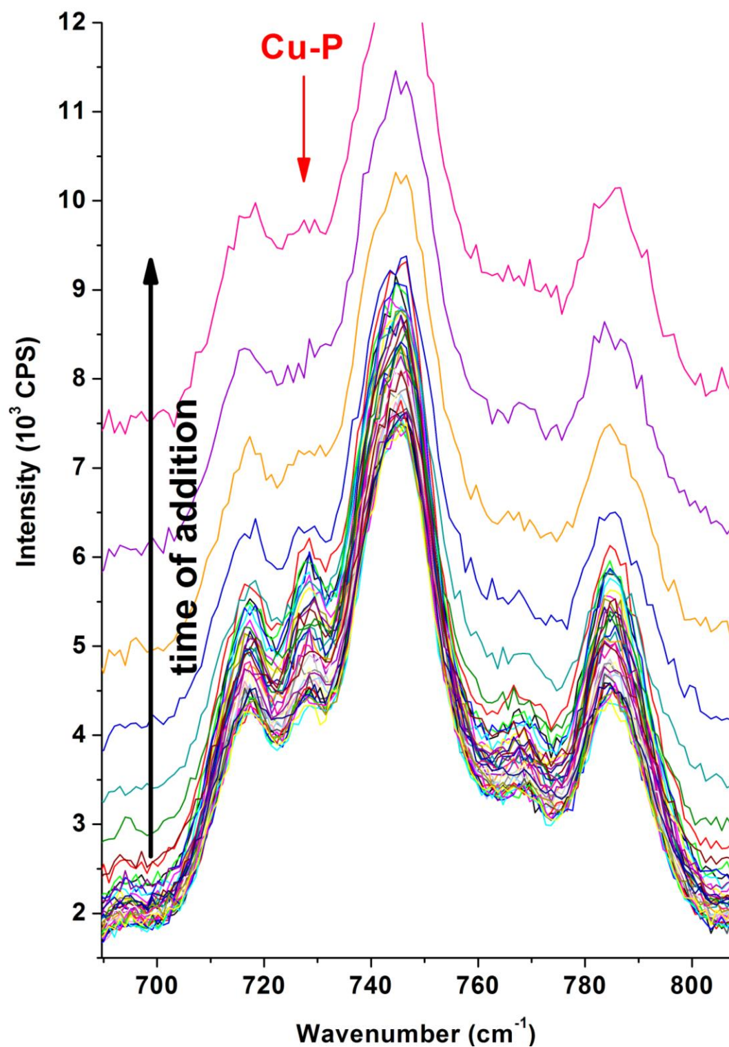
S 5. Variation of the Cu-P peak of a 0.0575 M In-TPP and Cu-TPP solution during the addition of a 0.1138 M hexamethyldisilathiane solution in acetonitrile ( 0.08 \text{ mL min}^{-1} ).
