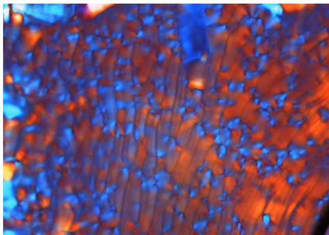
Figure A. The optical texture of C 18 E 3 in PAN at 25°C.
