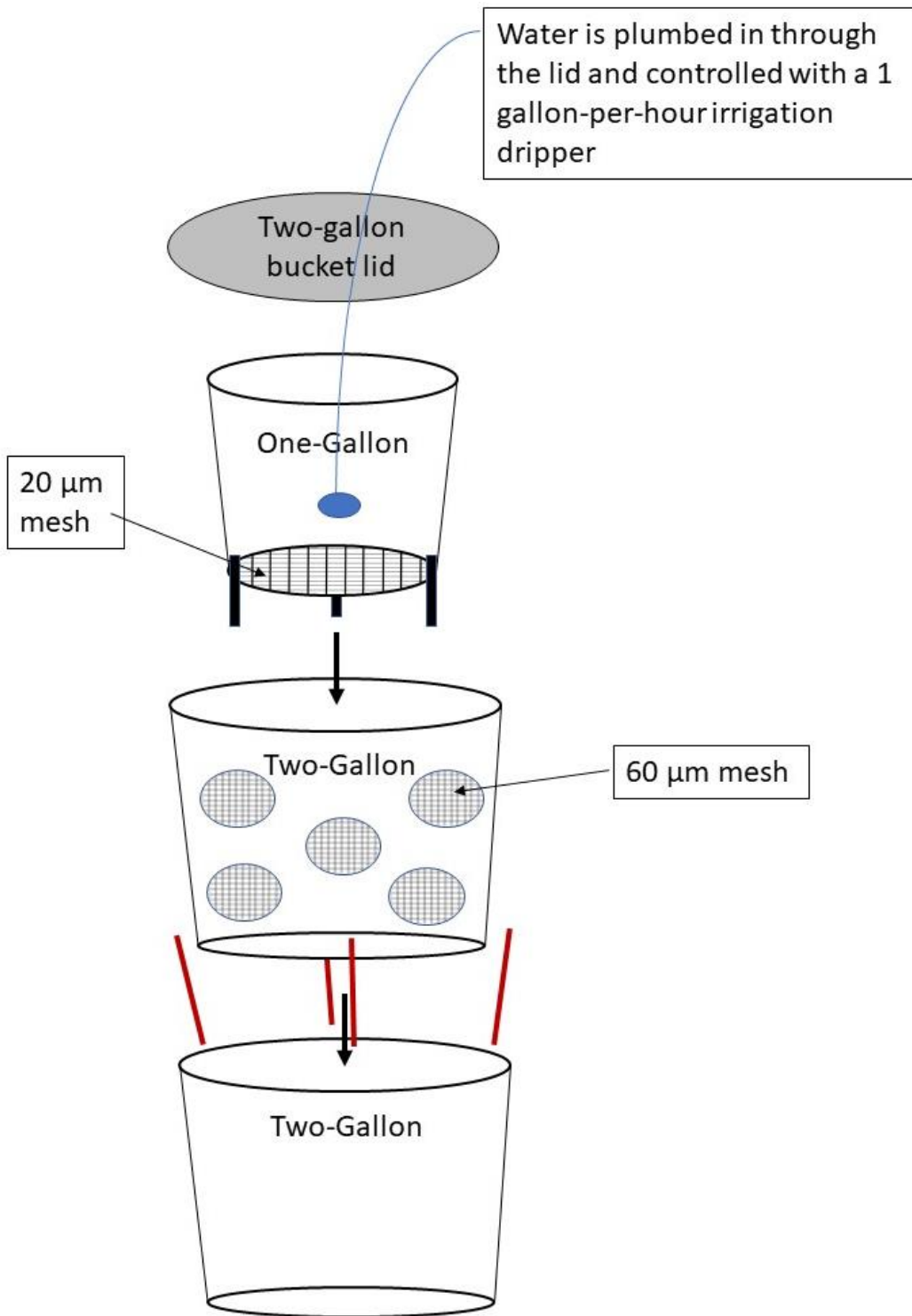
Figure S1. A schematic showing the different components of culture vessel construction.
