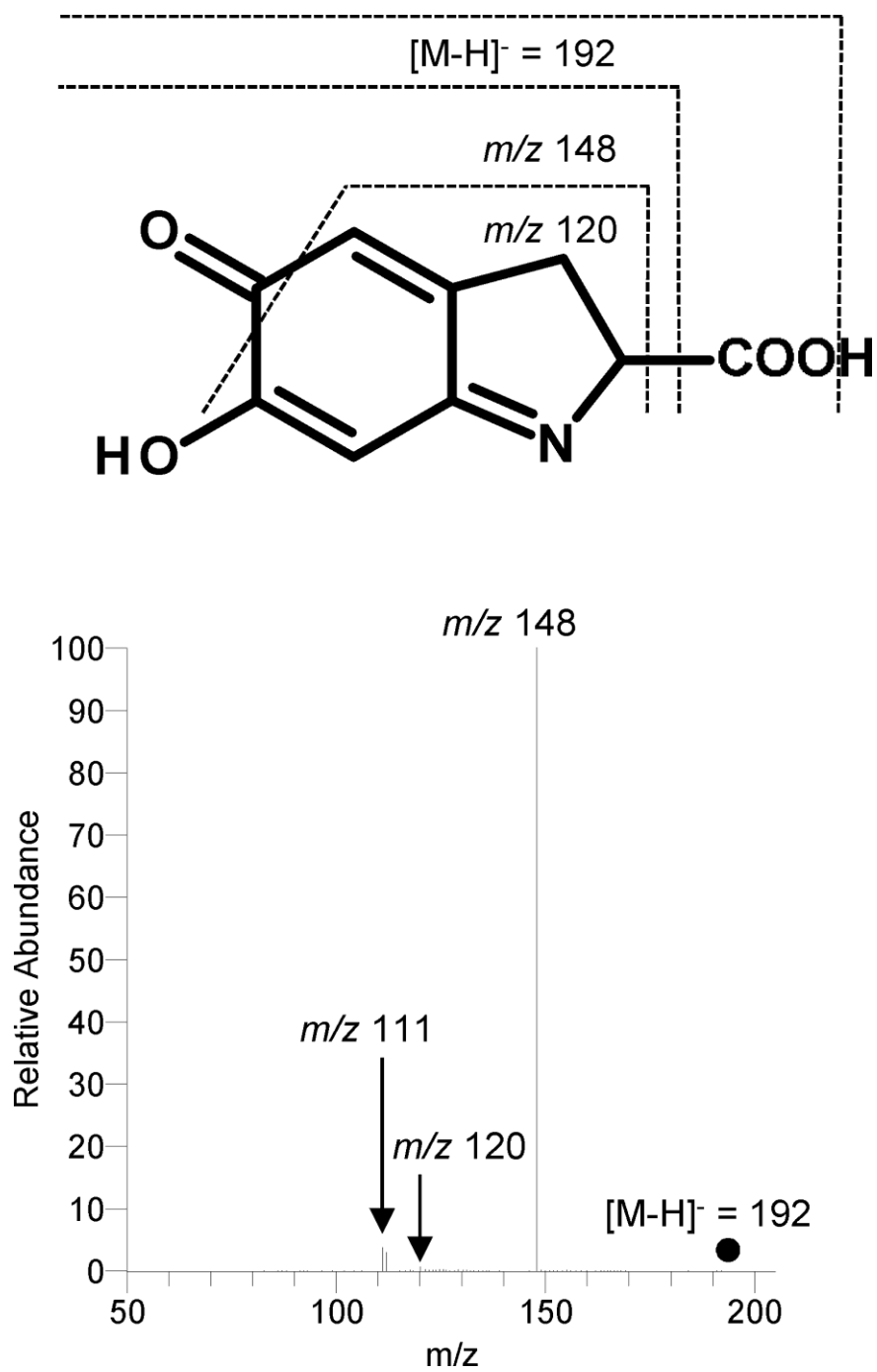
Figure S1. Fragmentation pattern of dopachrone in MS 2 .
