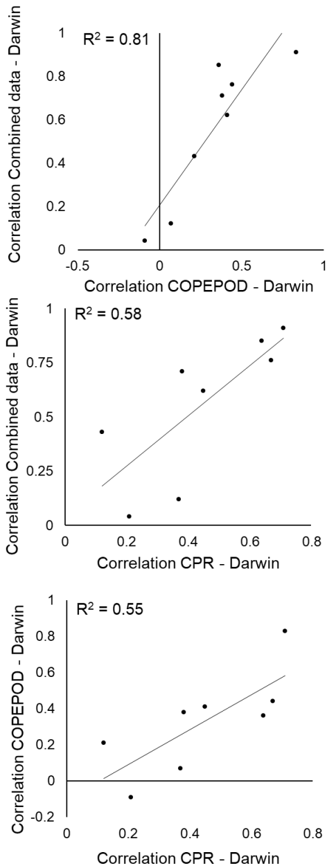
Supplementary Figure 1. A linear regression showing the relationship between the Pearson correlation coefficients between data and the model for each partition using the combined dataset and COPEPOD data only (top panel), combined dataset and CPR data only (middle panel) and the COPEPOD and CPR dataset (bottom panel). The R^2 for each regression are also shown within each panel.
