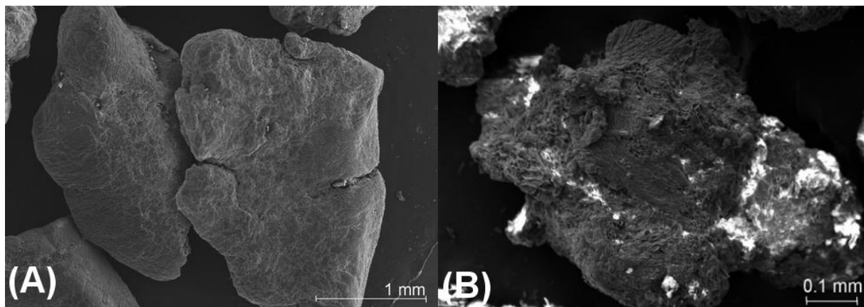
Fig. 2. SEM photographs of soybean meal (a) before biosorption, (b) Cr-loaded
