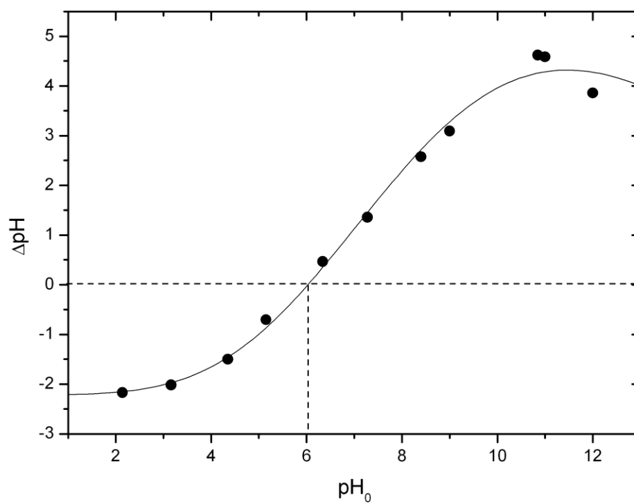
Fig. 3. pHzpc determination plot
