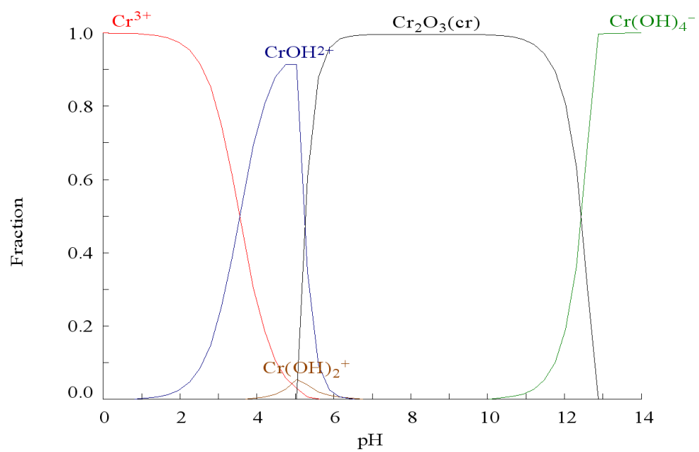
Fig. 4. Cr(III)-H 2 O diagram
