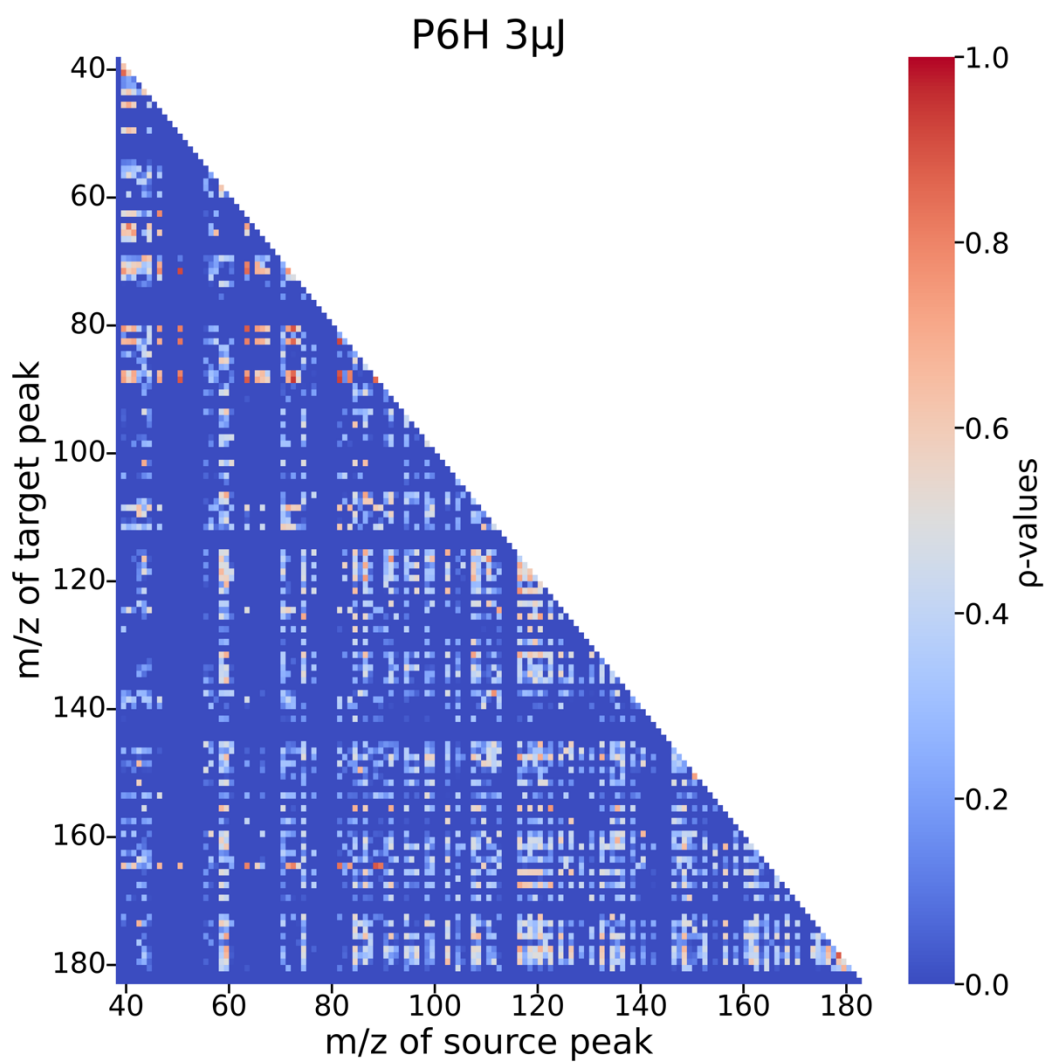
Figure 1 : Heatmap of the p-values from the amino acid extract of the P6H permafrost sample. As can be seen it is very hard to get information out of such a complex heatmap, which is another reason why correlation network analysis is a very good alternative to this analysis method.
