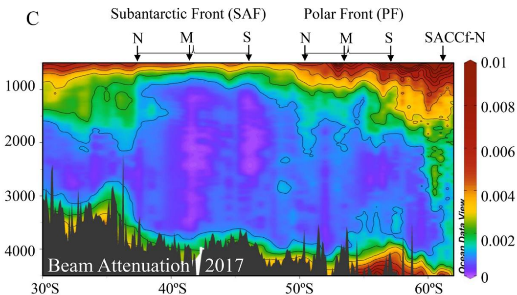
Figure S2. Beam attenuation distribution along P18 2017 transect [ \text{m}^{-1} ]. Note non-linear color bar.
