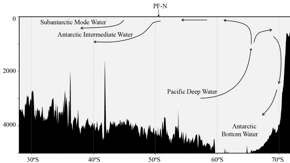
Figure S1. Large-scale overturning circulation and formation of major water masses in the Pacific sector of the Southern Ocean (derived from Talley et al., 2007 and Carter et al., 2022).
