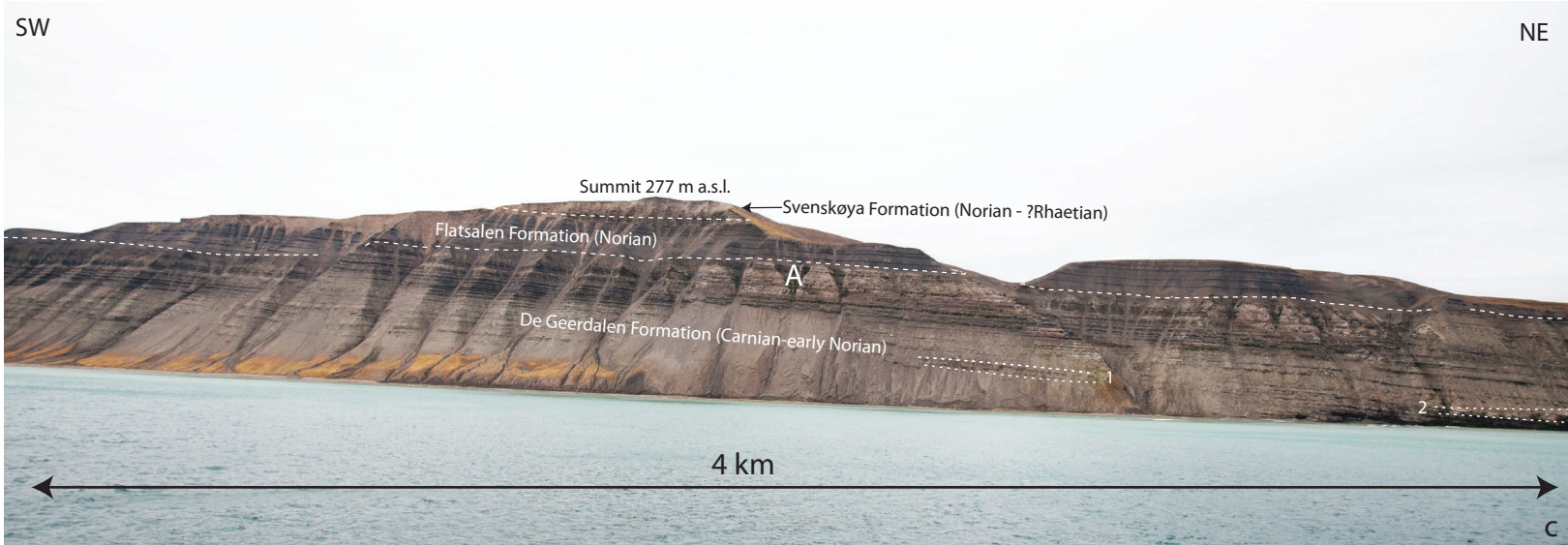
(c) The Upper Triassic north westward prograding delta of the De Geerdalen Formation in lower part is passing upward to offshore deposits of the Flatsalen Formation) and capped by mixed tidal fluvial channels of the The Svenskøya Formation). The deltaic De Geerdalen Formation consists of meandering fluvial channels, i.e., trunk rivers; 1 and 2 in the photo and overbank deposits.. South coast of the north-east part of Hopen.
