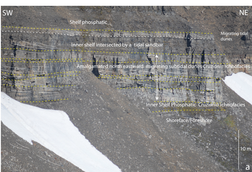
(a): Anisian north-eastward prograding coarse grained siliclastic wedge. The lower part consists of fine-grained sandstone representing shoreline deposits followed by offshore condensed phosphatic mudstone. Medium to very coarse grained quartz arenites and rare gravel in the middle part are interpreted as northeastward migrating subaqueous tidal dunes. Ladinian offshore shelf phosphatic muds from the upper part of the Bravaisberget Formation define the flooding of the wedge. Karentoppen, Sørkapp, Spitsbergen. (b): Lower Triassic inner shelf deposits of the Vikinghøgda Formation at the base are overlain by Middle Triassic organic rich marine mudstone of the Botneheia Formation. The late Ladinian to Carnian upper part shows prodelta to delta plain deposits representing the north-eastward prograding delta. Blanknuten, West coast of Edegøya. MU.Mbr.: Muen Member; Bl. Mbr: Blanknuten Member
