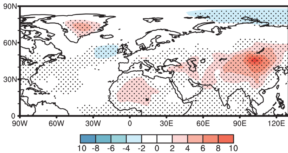
Figure S2 Regression coefficients of global temperature (index derived from https://climate.nasa.gov/vital-signs/global-temperature/ ) onto sea level pressure (shading, dots indicate significance at 90% confidence level according to the Student's- t test).
