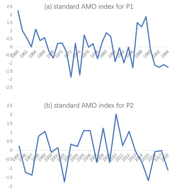
Figure S1 Standardized AMO index during (a) P1 and (b) P2, respectively.
