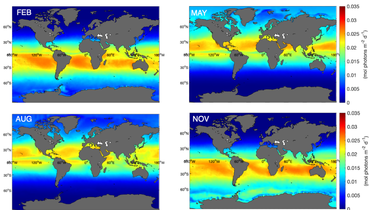
Supplementary Figure S1. Global maps of E_{CL,0}-(320\text{ nm}) in February, May, August and November. White color indicates no data.
