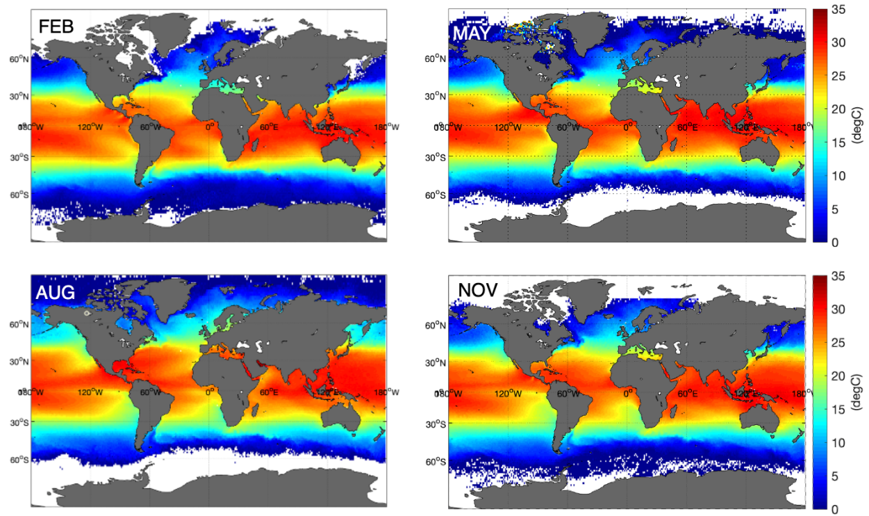
Supplementary Figure S4. Global maps of SST in February, May, August and November. White color indicates no data.
