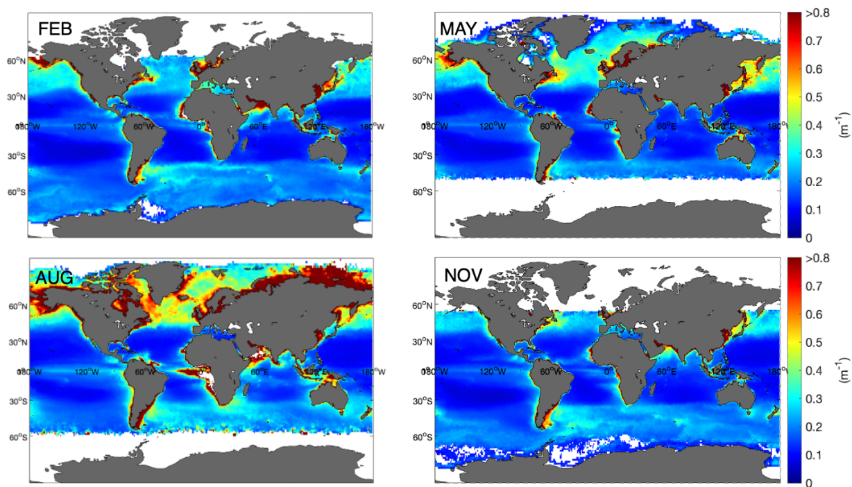
Supplementary Figure S3. Global maps of K_d(320 \text{ nm}) in February, May, August and November. White color indicates no data.
