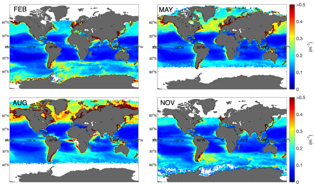
Supplementary Figure S2. Global maps of a_g(320 \text{ nm}) in February, May, August and November. White color indicates no data.
