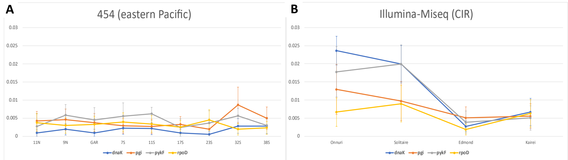
Supplementary Figure S1. Nucleotide diversity ( \pi ) of four genes for symbiotic bacteria. (A) dataset from 454 pyrosequencing. (B) dataset from Illumina-Miseq. The dot on the graph represents the mean of \pi for each gene and the vertical line above it represents the standard deviation computed from Arlequin v. 3.5.
