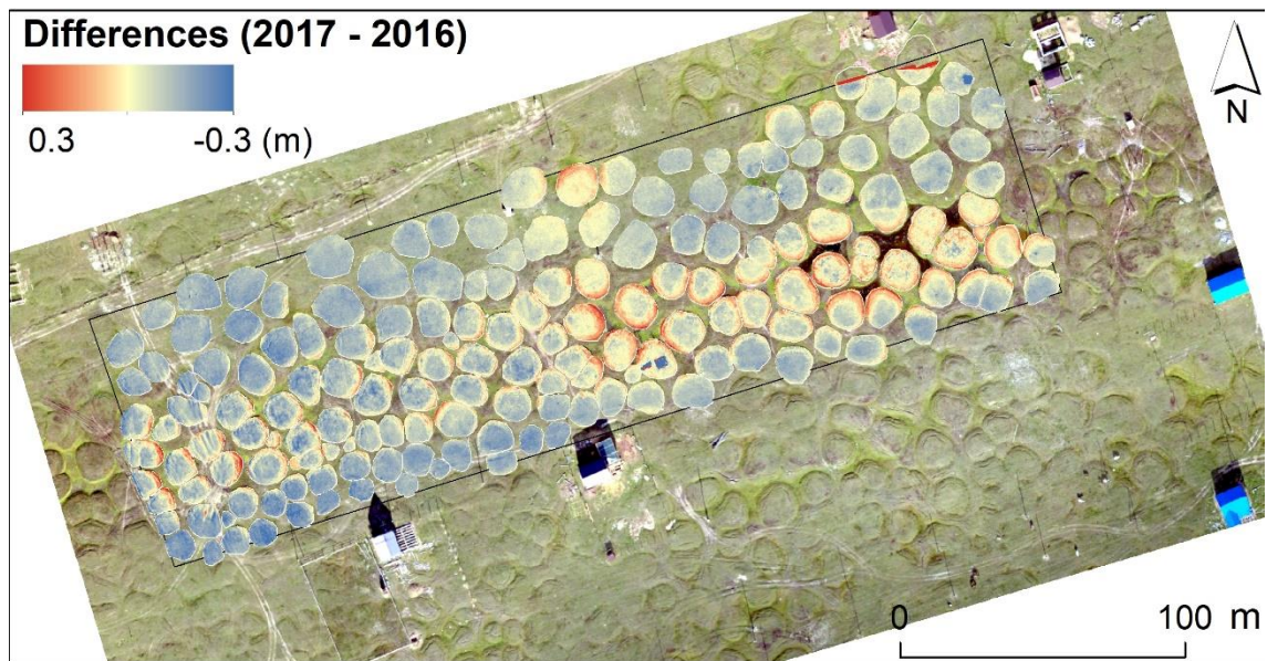
Figure S2: Difference between 2016 and 2017 DSMs. The difference was calculated only for the central part of the high-centered polygon.
