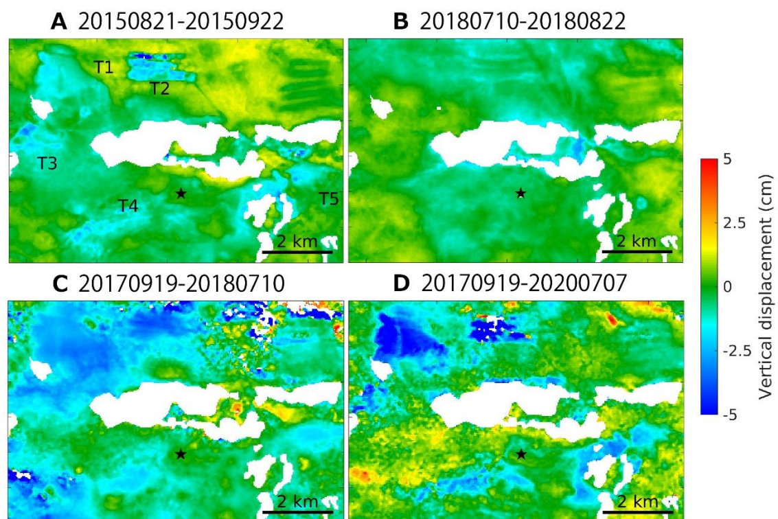
Figure S3: Some interferograms in which the image acquisition period of the pair was during (a and b) the same year, (c) one year and (d) three years.
