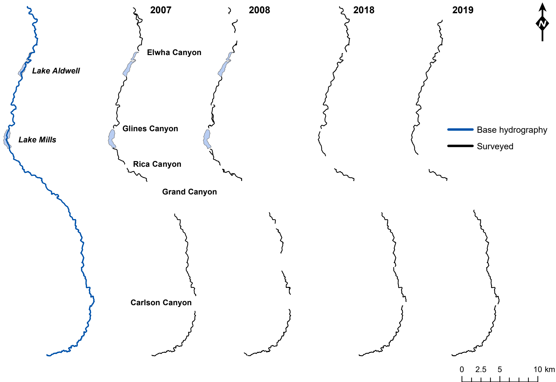
Figure S1. Reaches surveyed during riverscape study of salmonid distribution and abundance during base flow conditions before (2007, 2008) and after (2018, 2019) dam removal in the Elwha River, Washington, USA. Base hydrography (stream line) depicted on left was derived from high-resolution (< 1 m) aerial photographs collected in 2017.
