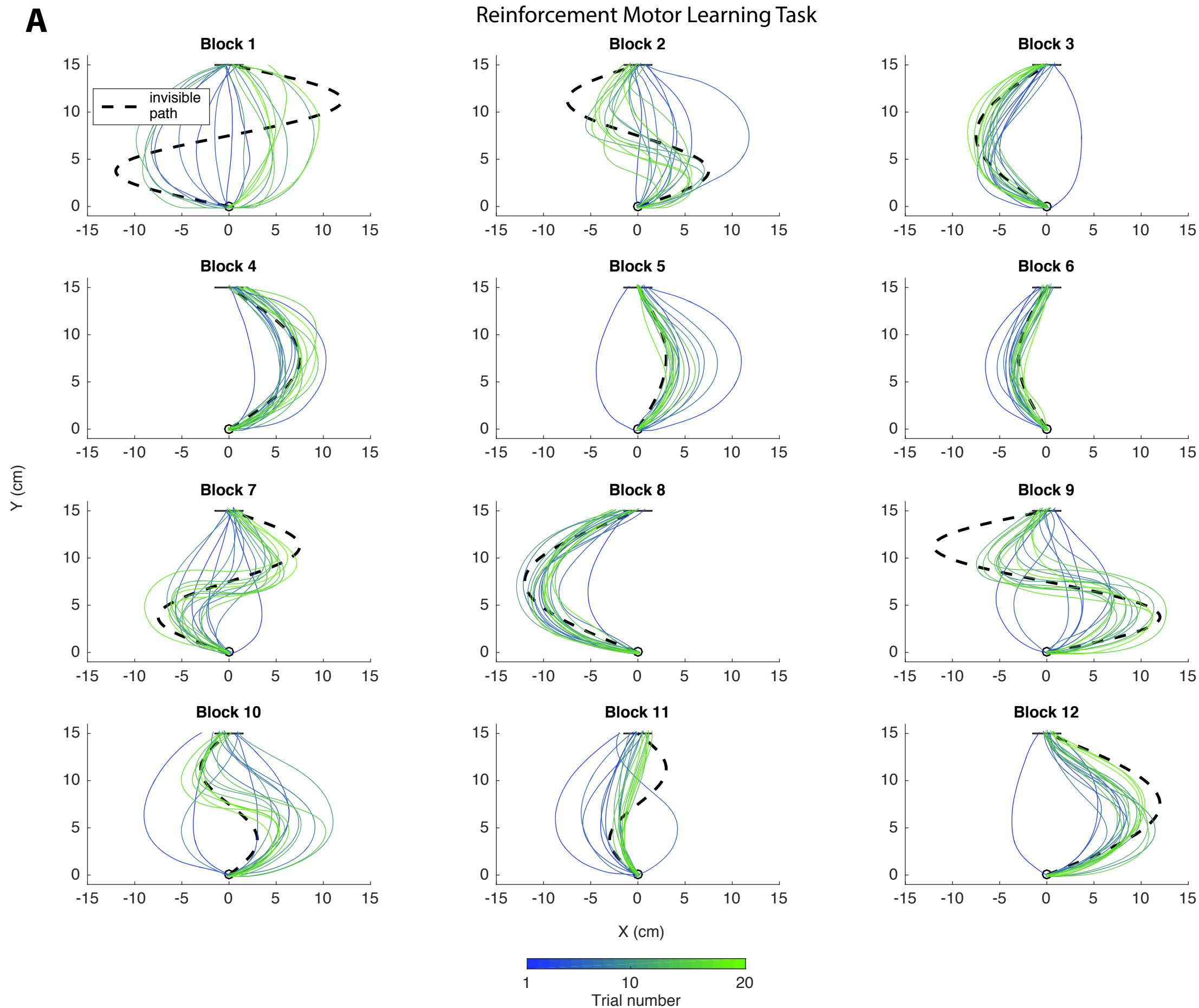
Figure Caption: Motor learning data for subject 16 (S16). (A) Path trajectories in the Reinforcement motor learning task for each trial block. Trajectories are color-coded (from blue to green) based on trial number (see color legend at bottom). (B) Reach angles in the Error-based learning task plotted as a function of trial number. Blue data points indicate reach movements whereas purple data points indicate the subject's reported aiming direction. Red horizontal line denotes full compensation for the visuomotor rotation. (C) Distribution of scores for single and double curve performance in the reinforcement motor learning task, and distrubtion of angular errors and reported aiming direction errors in the error-based motor learning task. Each dot indicates the mean value of one participant and the horizontal line indicates the mean across participants, and the shaded area indicates the standard error of the mean. Larger black dots denote the data belonging to this particular subject.
