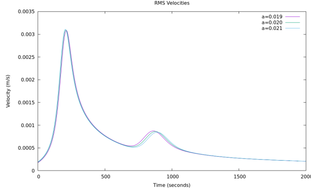
Figure 78: Computations of the van Keken problem made with the VOF interface tracking algorithm showing the evolution of the RMS velocity as a function of time for small changes in the amplitude a of the cosine function in the initial condition at 7 levels of refinement. Compare to Figures 72 and 76.
