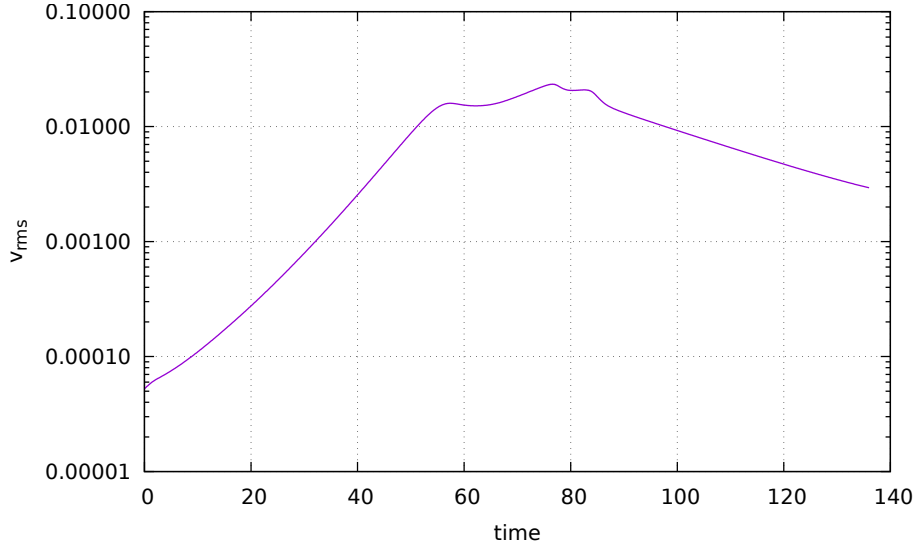
Figure 84: Polydiapirism benchmark: Root mean square velocity as a function of time
