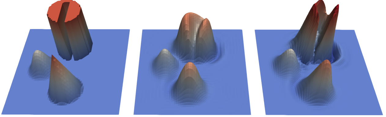
Figure 121: Rotating shapes benchmark at final time: Left: reference. Middle: Entropy viscosity. Right: SUPG.
