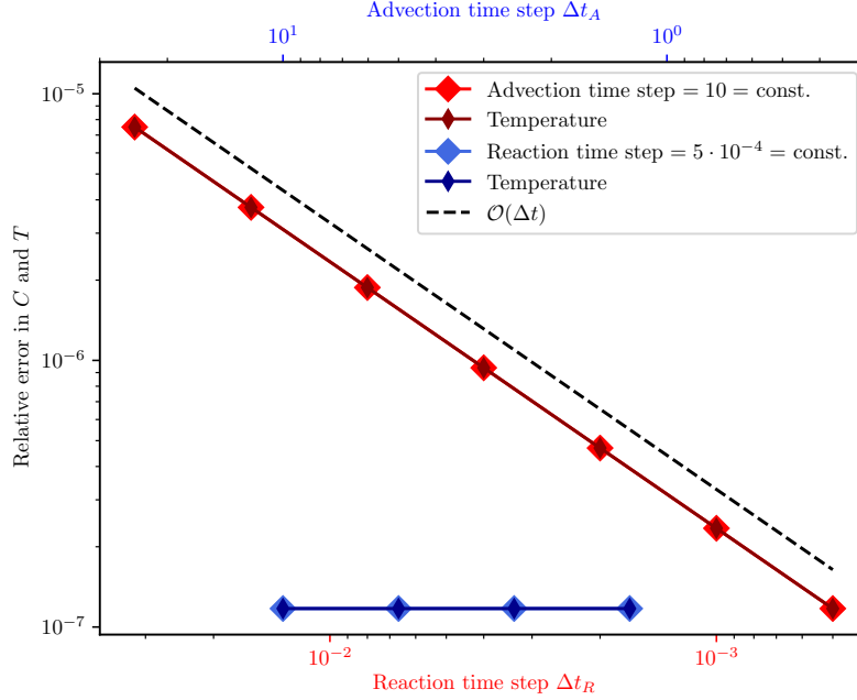
Figure 114: Error for both compositional field and temperature compared to the analytical solution, varying the time steps of advection (blue data points and top/blue x axis) and reactions (red data points and bottom/red x axis), while keeping the other one constant, respectively.
