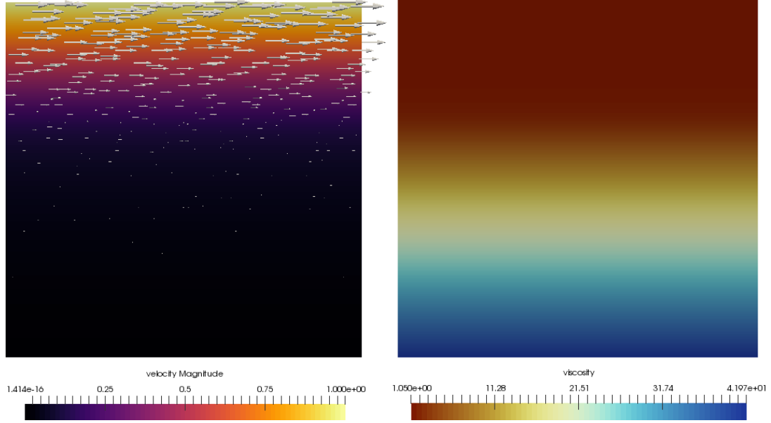
Figure 118: Velocity and viscosity fields for \beta = 0.01 and \epsilon = 0.05 at uniform level 8 resolution, using y_0 = 1/3 .
