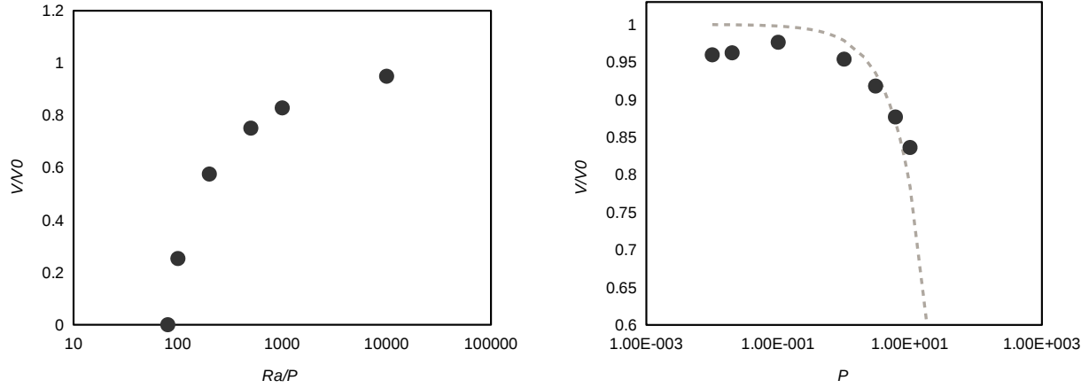
Figure 61: Translation rate (approximated by the average of the velocity component in the direction of translation), normalized to the low \mathcal{P} limit estimate given in [36], as a function of \frac{Ra}{\mathcal{P}} for \mathcal{P} = 10^{-2} (left) and as a function of \mathcal{P} for Ra = 10^5 (right). The dashed gray line gives the translation velocity predicted in the limit of low \mathcal{P} . Disagreement for larger values of \mathcal{P} indicates that higher order terms (not included in the low \mathcal{P} approximation) become important. Additionally, differences between the analytical and numerical model might be the result of limited resolution (only 12 elements in radial direction).
