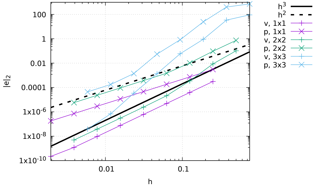
Figure 103: Viscosity grooves benchmark: Velocity and pressure error convergence as a function of the mesh size h for 3 domain sizes.
