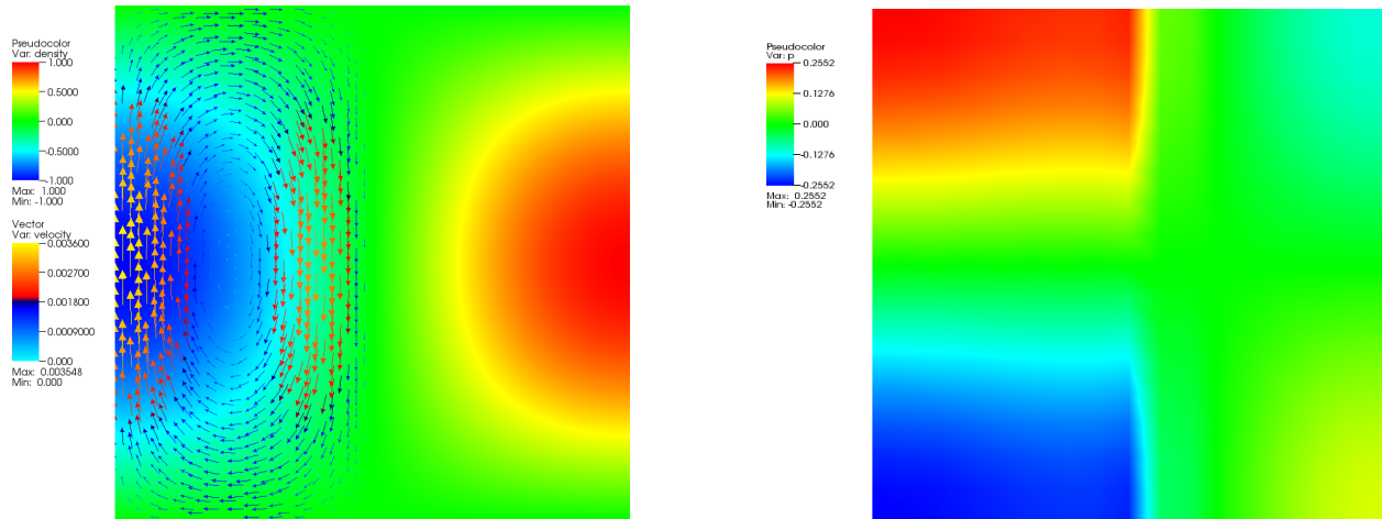
Figure 87: SolCx Stokes benchmark. Left: The density perturbation field and overlaid to it some velocity vectors. The viscosity is very large in the right hand, leading to a stagnant flow in this region. Right: The pressure on a relatively coarse mesh, showing the internal layer along the line where the viscosity jumps.
