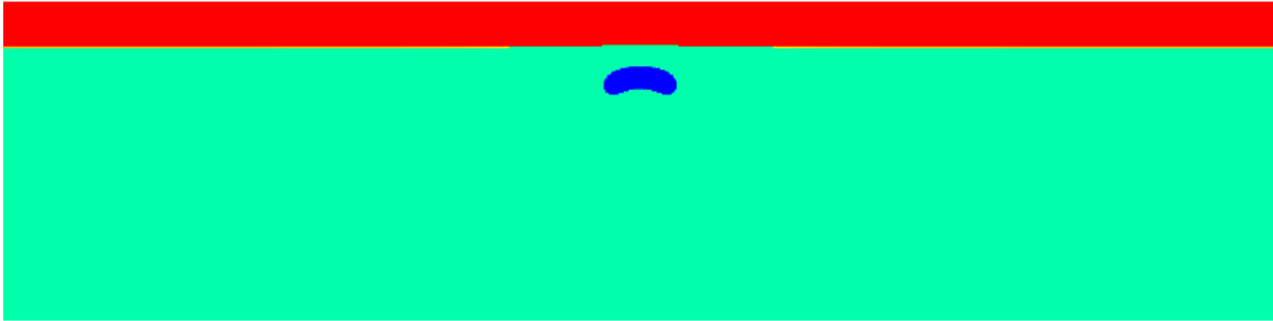
Figure 110: Setup for the dynamic topography benchmark. Again, the domain is 2800 km wide and 700 km high. A 100 km thick lid with viscosity 10^{23} overlies a mantle with viscosity 10^{21} . Both the lid and the mantle have a density of 3300 \text{ kg/m}^3 . A blob with diameter 100 km lies 300 km from the bottom of the domain. The blob has a density of 3200 \text{ kg/m}^3 and a viscosity of 10^{20} \text{ Pa s} .
