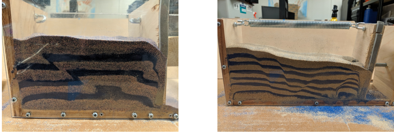
Figure 123: Examples of deformation patterns of “sand box” experiments in which alternating layers of differently-colored sand undergo deformation. Pictures courtesy of the lab of Dennis Harry at Colorado State University.
