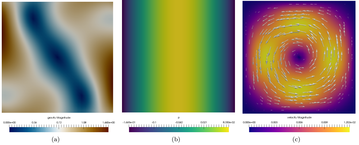
Figure 119: Donea & Huerta benchmark: Results for the 2D polynomial Stokes benchmark, obtained with a resolution of 32 \times 32 elements. (a) Gravity field, (b) pressure field, (c) velocity field.
