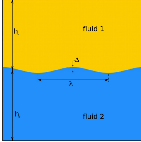
Figure 80: Setup of the Rayleigh-Taylor instability benchmark (taken from [96])
