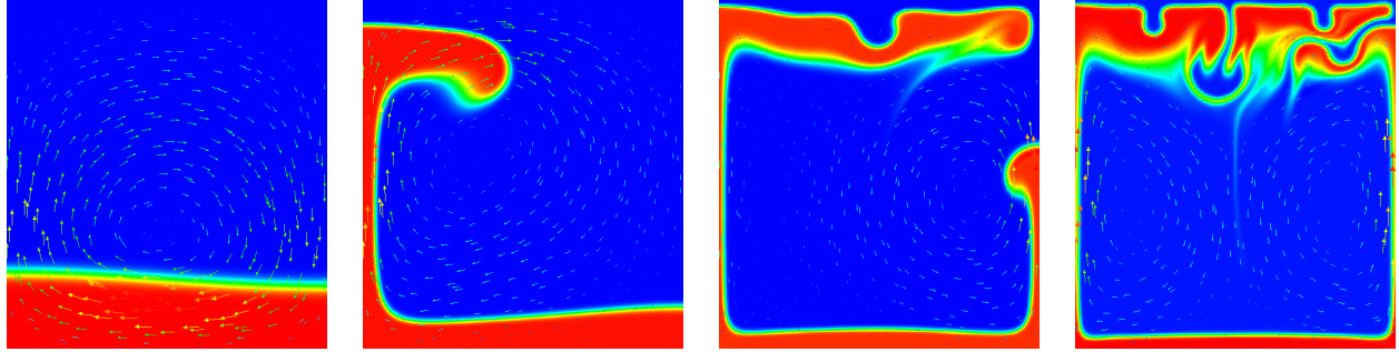
Figure 67: Van Keken benchmark (using a smoothed out interface, see the main text): Compositional field at times t = 0, 300, 900, 1800 .
