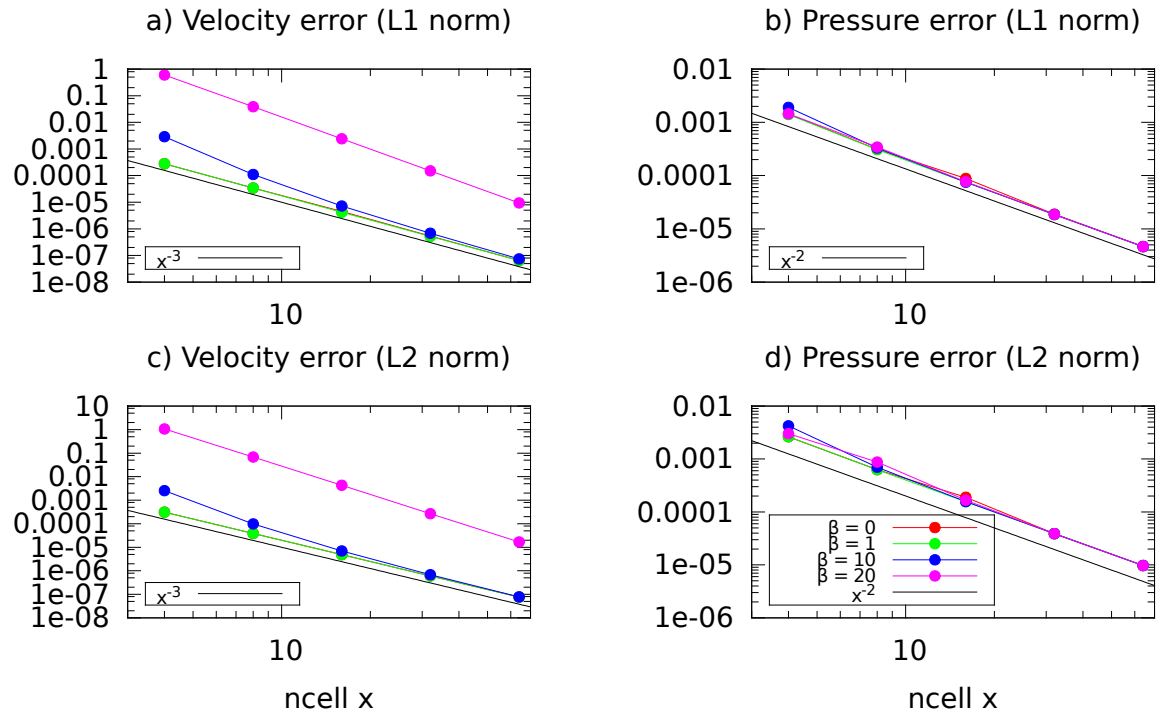
Figure 92: Burstedde benchmark: Error convergence for the 3D polynomial Stokes benchmark.
