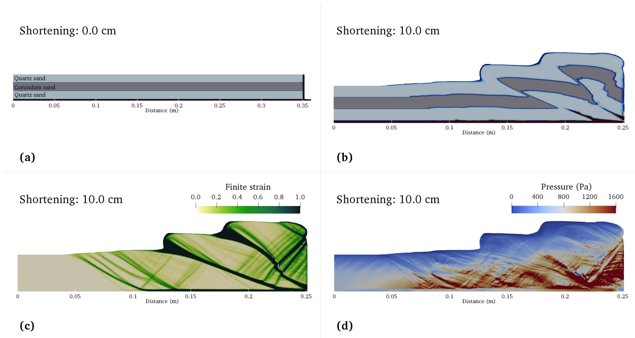
Figure 125: Numerical model of an unstable subcritical wedge. a) Initial model setup. b) Material field of sands after 10 cm shortening. c) Strain field and d) pressure field.
