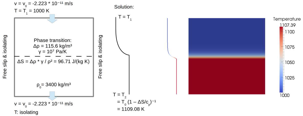
Figure 104: Latent heat benchmark. Both figures show the 2D box model domain. Left: Setup of the benchmark together with a sketch of the expected temperature profile across the phase transition. The dashed line marks the phase transition. Material flows in with a prescribed temperature and velocity at the top, crosses the phase transition in the center and flows out at the bottom. The predicted bottom temperature is T_2 = 1109.08 K. Right: Temperature distribution of the model together with the associated temperature profile across the phase transition. The modelled bottom temperature is T_2 = 1107.39 K.
