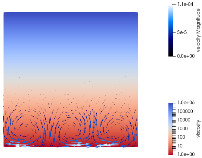
Figure 89: SolKz Stokes benchmark. Another view of the velocity vectors, this time plotted over the viscosity field.
