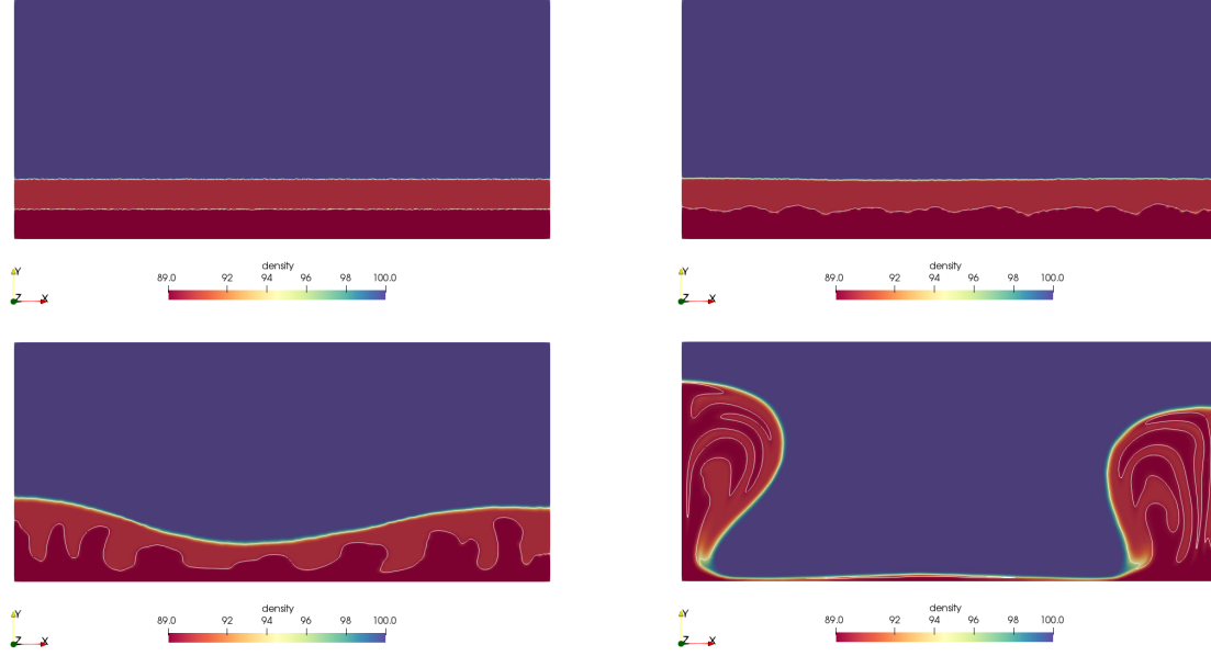
Figure 83: Polydiapirism benchmark: Density field at t = 0, 25, 50, 75 s.
