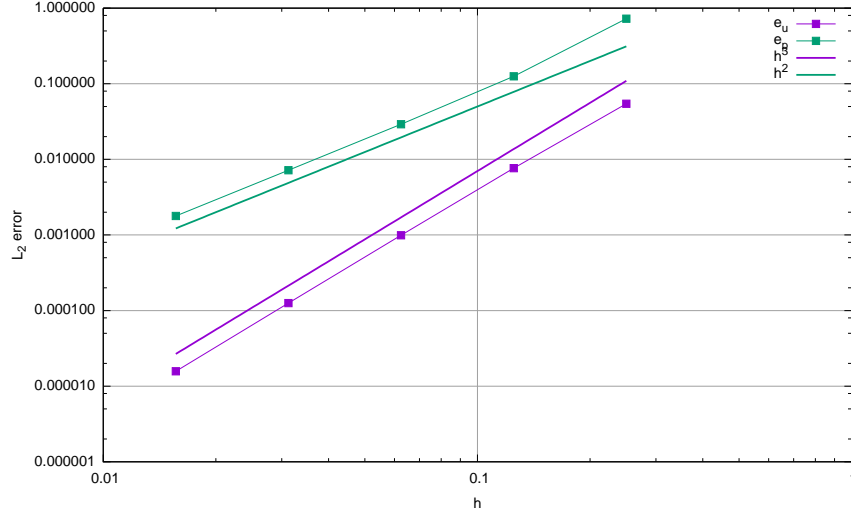
Figure 96: Velocity and pressure errors in the L_2 -norm as a function of the mesh size.
