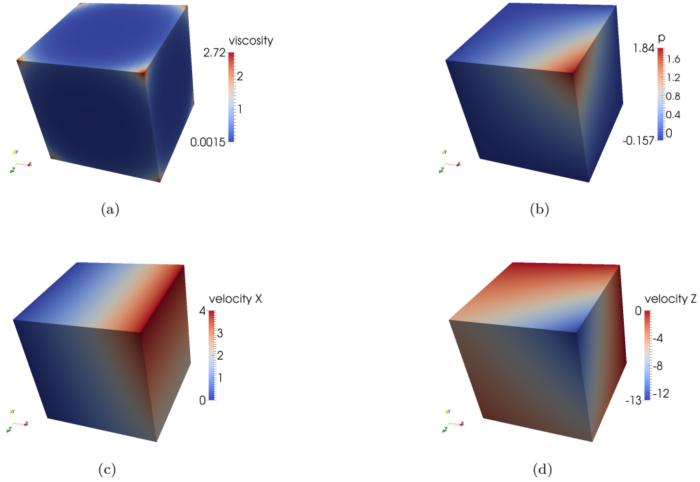
Figure 91: Burstedde benchmark: Results for the 3D polynomial Stokes benchmark, obtained with a resolution of 16 \times 16 elements, with \beta = 10 .
