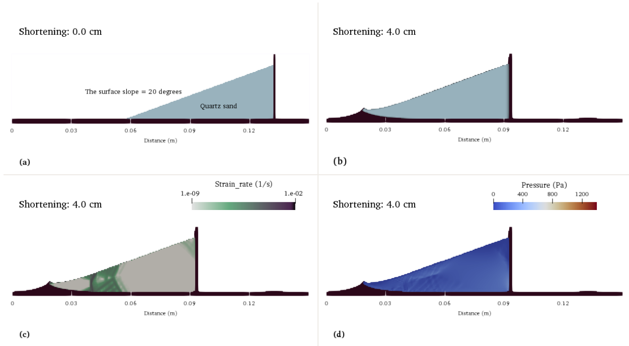
Figure 124: Numerical model of a stable sand wedge. a) Initial model setup. b) Material field after 4 cm of translation. c) Strain rate field and d) pressure field.
