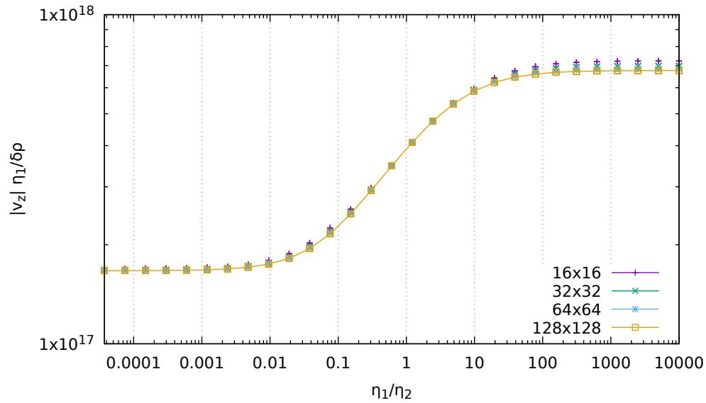
Figure 86: Scaled velocity measurements as a function of the viscosity contrast between surrounding medium and block for all experiments.
