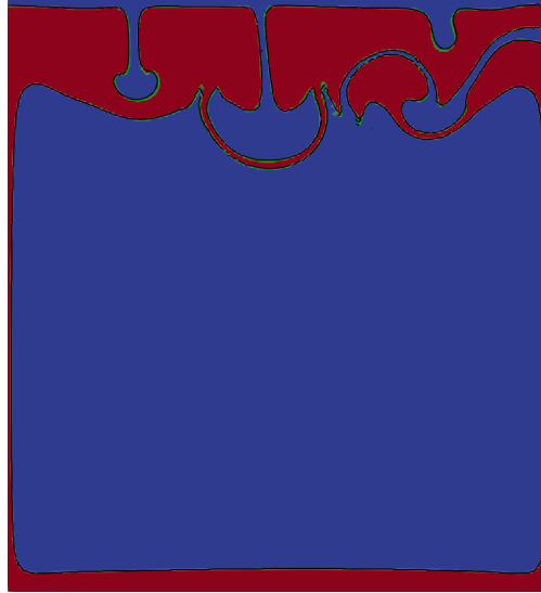
Figure 77: The results of two computations of the van Keken problem made with the VOF interface tracking algorithm overlaid upon each other at t_{\text{end}} = 2000 . This visualization shows the reconstructed boundary between the two materials at the final time t_{\text{end}} as computed on a uniform grid with 7 and 8 levels of refinement. The boundaries between the materials are displayed as contours of the fields \psi^7(t_{\text{end}}) (black) and \psi^8(t_{\text{end}}) (bright green), which are generated by the visualization postprocessor. The contours for the reconstructed material boundaries are superimposed on a color gradient visualization of the material composition for the computation with 8 levels of refinement in order to make the regions with each fluid type more evident. Compare with the fourth image on the right in Figure 67.
