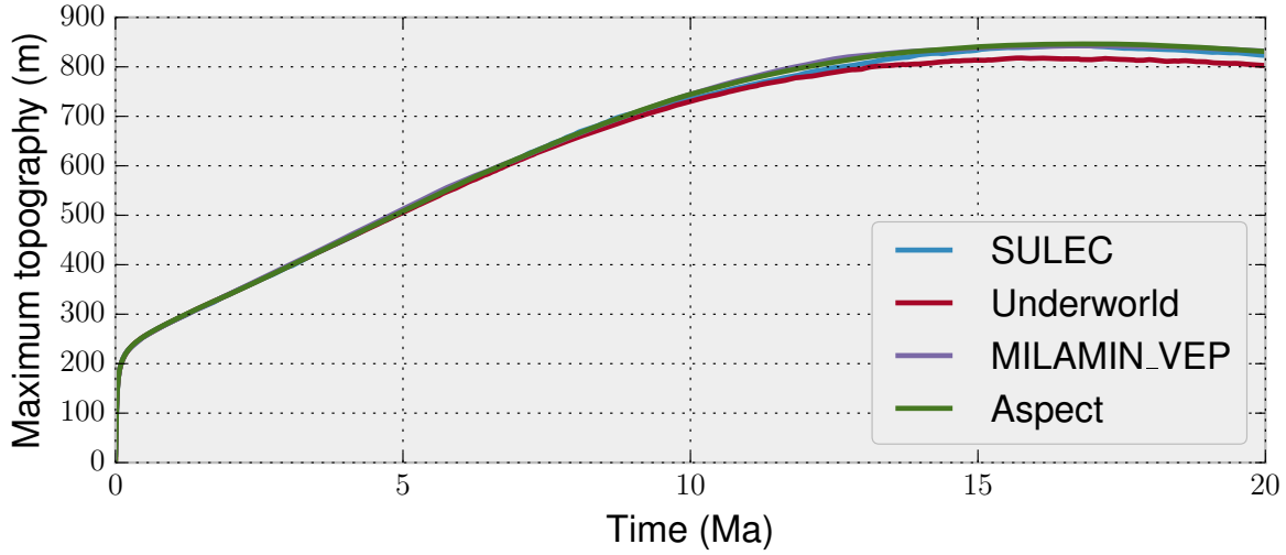
Figure 111: Evolution of topography for the dynamic topography benchmark. The maximum topography is shown as a function of time, for ASPECT as well as for several other codes participating in the benchmark. This benchmark shows considerably more scatter between the codes.
