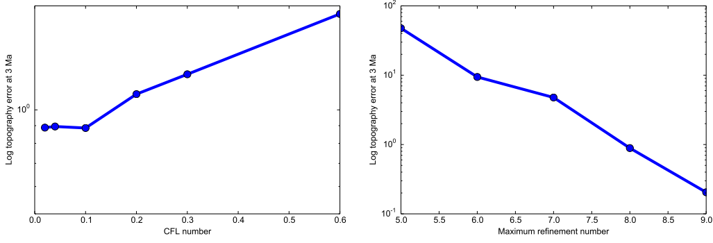
Figure 112: Convergence for case two. Left: Logarithm of the error with decreasing CFL number. As the CFL number decreases, the error gets smaller. However, once it reaches a value of \sim 0.1 , there stops being much improvement in accuracy. Right: Logarithm of the error with increasing maximum mesh resolution. As the resolution increases, so does the accuracy.
