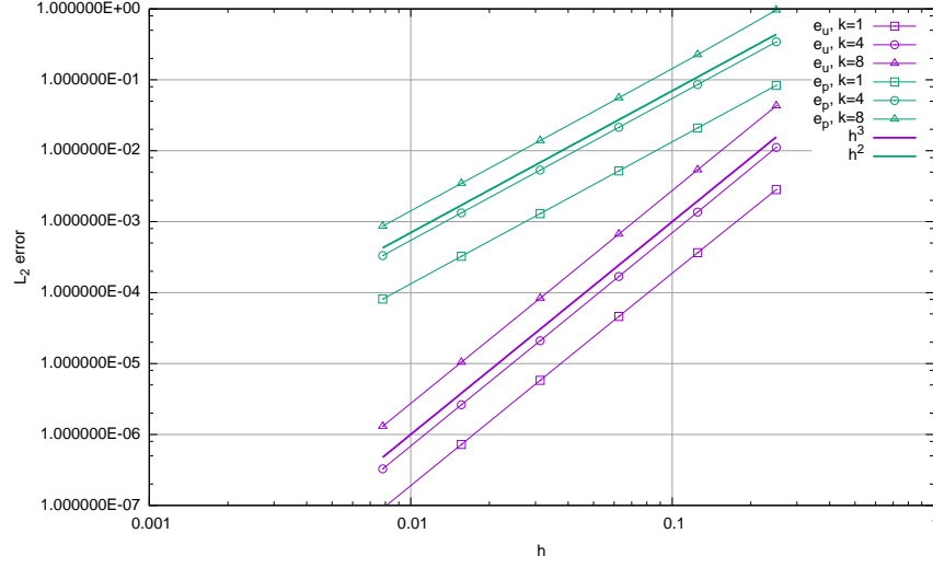
Figure 98: Velocity and pressure errors in the L_2 -norm as a function of the mesh size for the 2D annulus benchmark.
