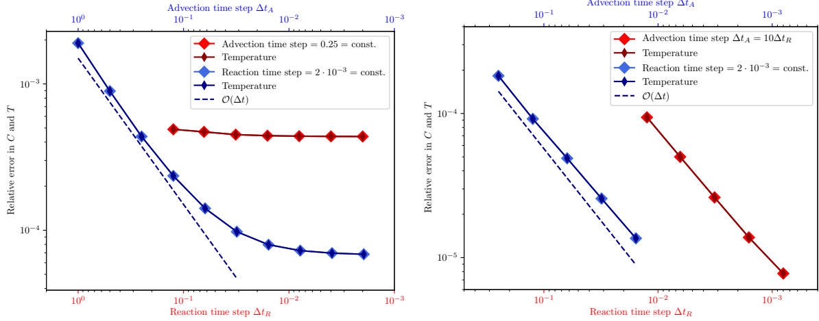
Figure 115: Error for both compositional field and temperature compared to the analytical solution, varying the time steps of advection (blue data points and top/blue x axis) and reactions (red data points and bottom/red x axis), while keeping the other one constant, respectively.
