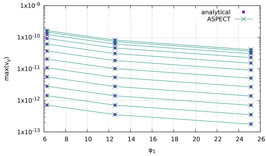
Figure 82: Maximum velocity for three values of the \phi_1 parameter.
