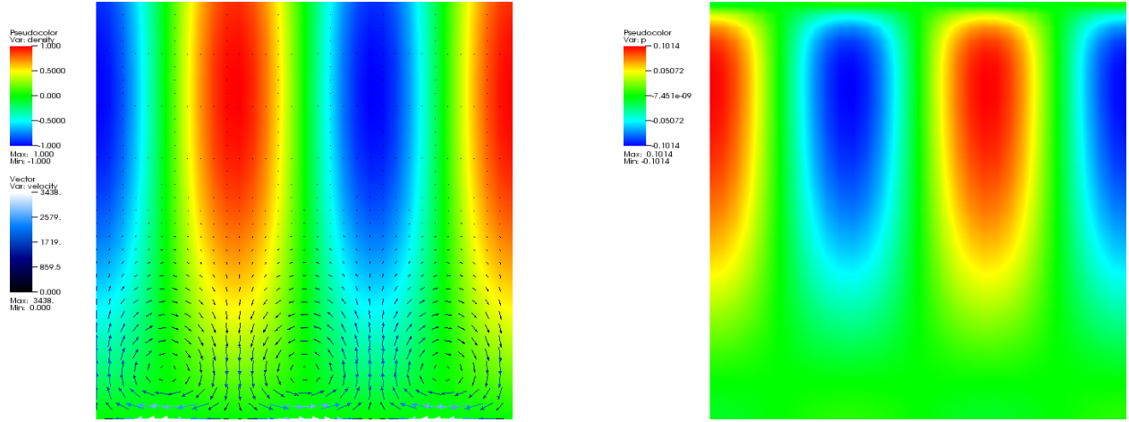
Figure 88: SolKz Stokes benchmark. Left: The density perturbation field overlaid with velocity vectors. The viscosity grows exponentially in the vertical direction, leading to small velocities at the top despite the large density variations. Right: The pressure.
