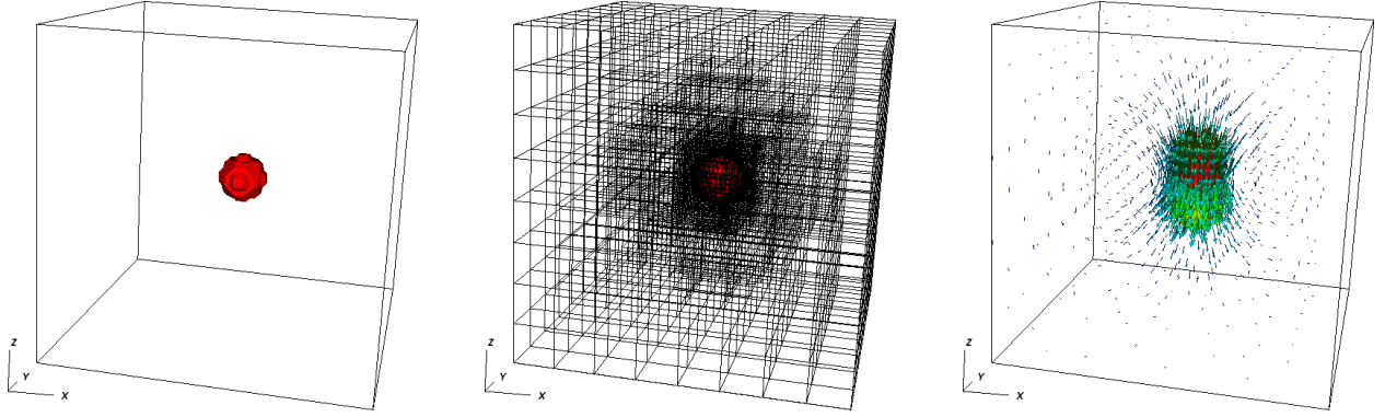
Figure 100: Stokes benchmark. Three-dimensional views of the compositional field (left), the adaptively refined mesh (center) and the resulting velocity field (right).
