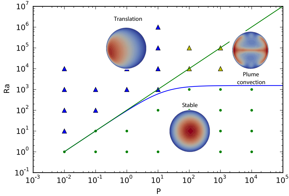
Figure 59: Stability diagram for convection in a sphere with phase change at its outer boundary. The stability curves for the first unstable mode ( l=1 ) and the translation are obtained from [36]. Each dot (no convection) and triangle (blue: translation, yellow: plume convection) is one model run done with ASPECT. The highest the Ra and P are, the more refinement is required (see text).
