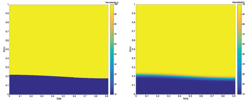
Figure 73: Van Keken benchmark using different-viscosity layers. The left image is the discontinuous case, while right is the smooth. Both are shown at t = 0 .
