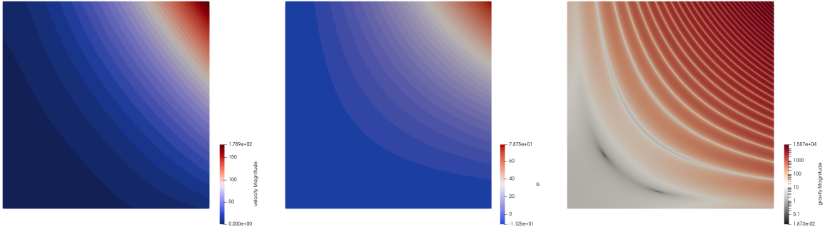
Figure 101: Viscosity grooves benchmark: From left to right, velocity field, pressure field, and norm of the right hand side of the momentum equation, for a 3 \times 3 domain with \epsilon = 0.1 .
