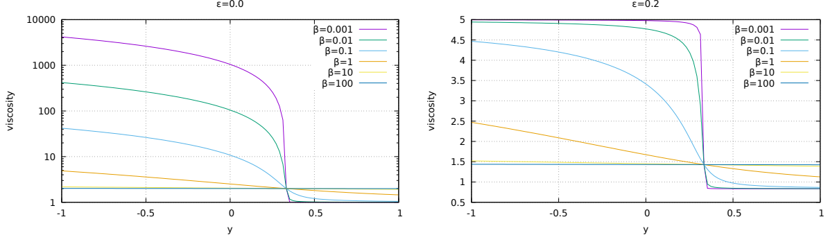
Figure 117: Layered flow benchmark: Viscosity profiles for various \beta values and two \epsilon values, using y_0 = 1/3 .
