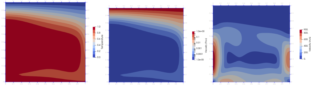
Figure 116: Temperature and viscosity field in steady-state for case 1 of [100].
