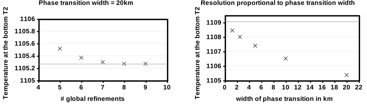
Figure 105: Results of the latent heat benchmark. Both figures show the modelled temperature T_2 at the bottom of the model domain. Left: T_2 in dependence of resolution using a constant phase transition width of 20 km. With an increasing number of global refinements of the mesh, the bottom temperature converges against a value of T_2 = 1105.27 K. Right: T_2 in dependence of phase transition width. The model resolution is chosen proportional to the phase transition width, starting with 5 global refinements for a width of 20 km. With decreasing phase transition width, T_2 approaches the theoretical value of 1109.08 K
