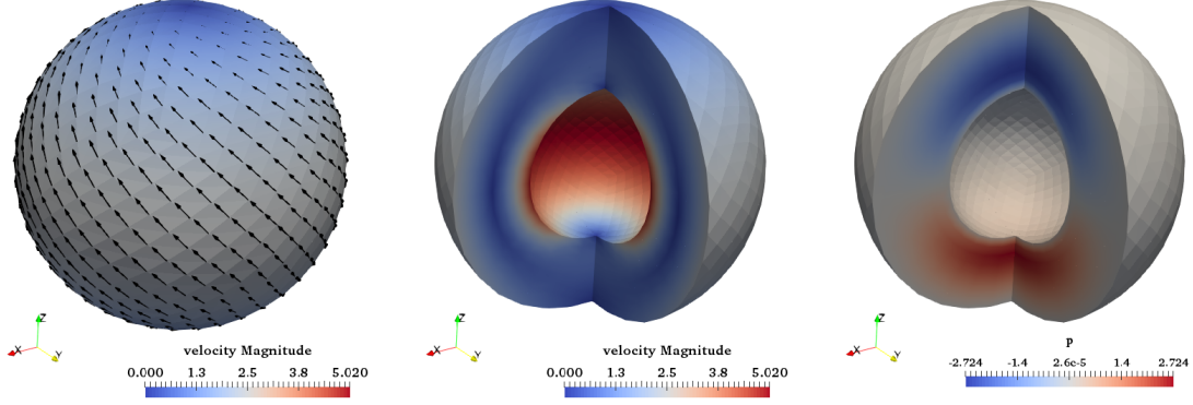
Figure 95: Velocity and pressure fields for the hollow sphere benchmark.
