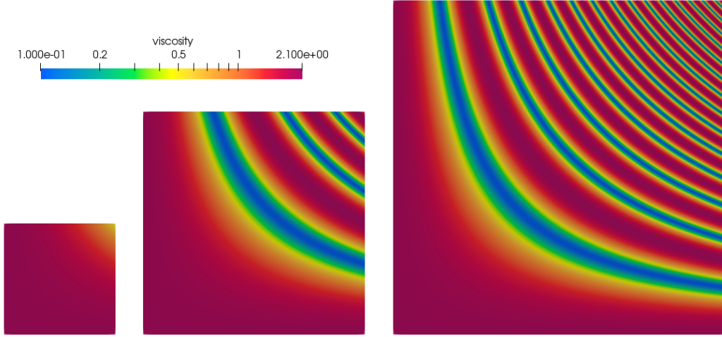
Figure 102: Viscosity grooves benchmark: Viscosity field for three domain sizes: 1 \times 1 , 2 \times 2 and 3 \times 3 .
