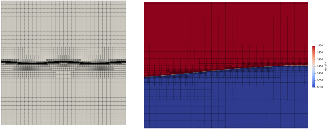
Figure 81: Left: grid with initial global refinement 4 and adaptive refinement 6; Right: density field with detail of the mesh.
