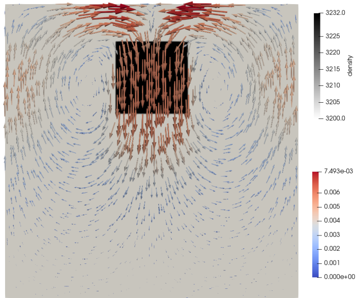
Figure 85: Density field with velocity arrows for \eta_2 = 10^{27} \text{ Pa s} and \delta\rho = 32 \text{ kg/m}^3
