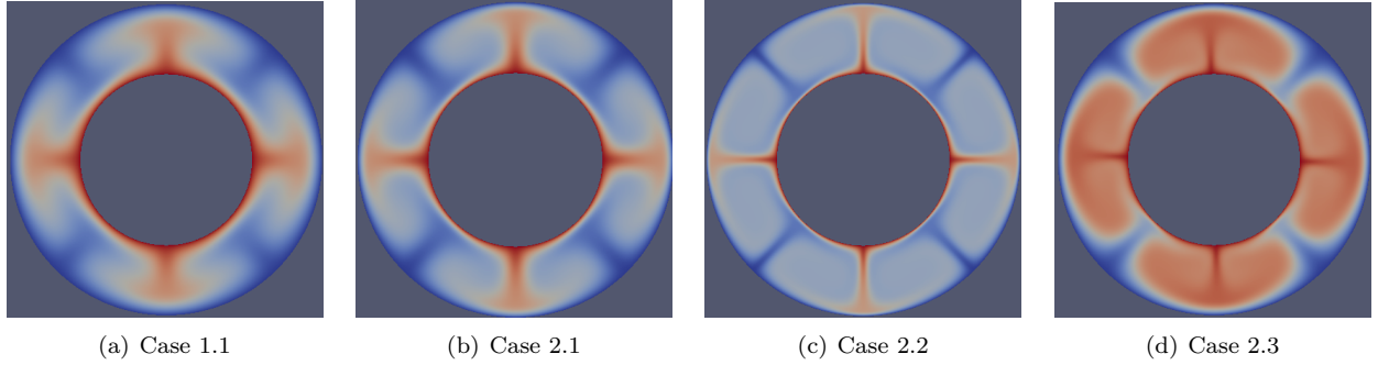
Figure 106: Davies et al. benchmarks: Final steady state temperature fields for the 2D cylindrical benchmark cases.
