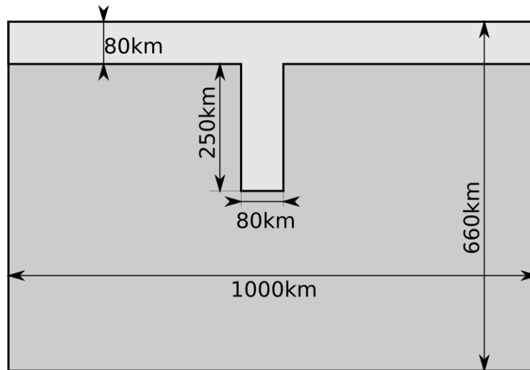
Figure 93: Slab detachment benchmark: Initial geometry
