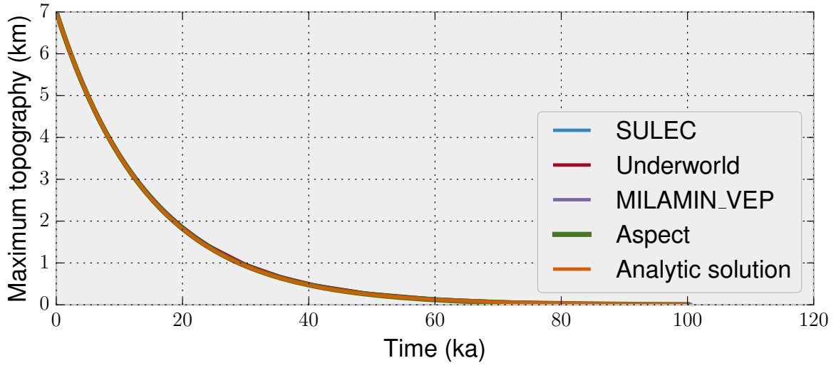
Figure 109: Results for the topography relaxation benchmark, showing maximum topography versus time. Over about 100 ka the topography completely disappears. The results of four free surface codes, as well as the semi-analytic solution, are nearly identical.
