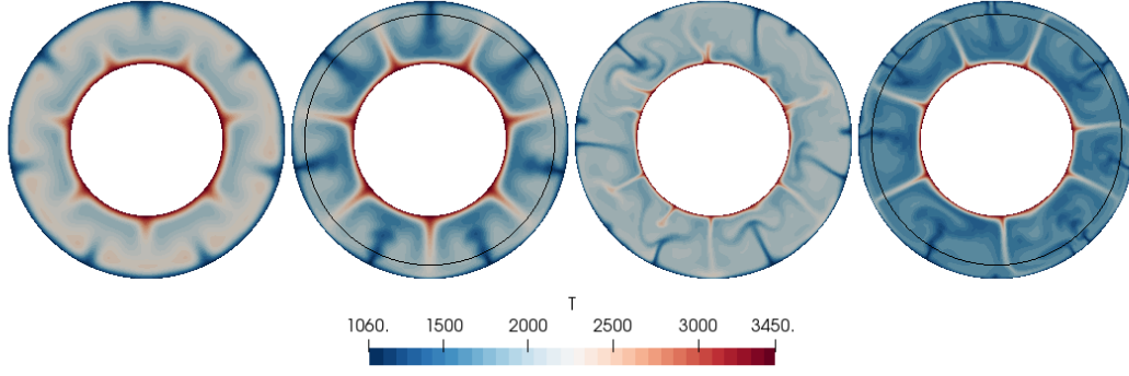
Figure 79: Bunge et al. benchmark. From left to right: temperature field at time t = 5 \cdot 10^9 years obtained with viscosity profiles a, b, c and d.
