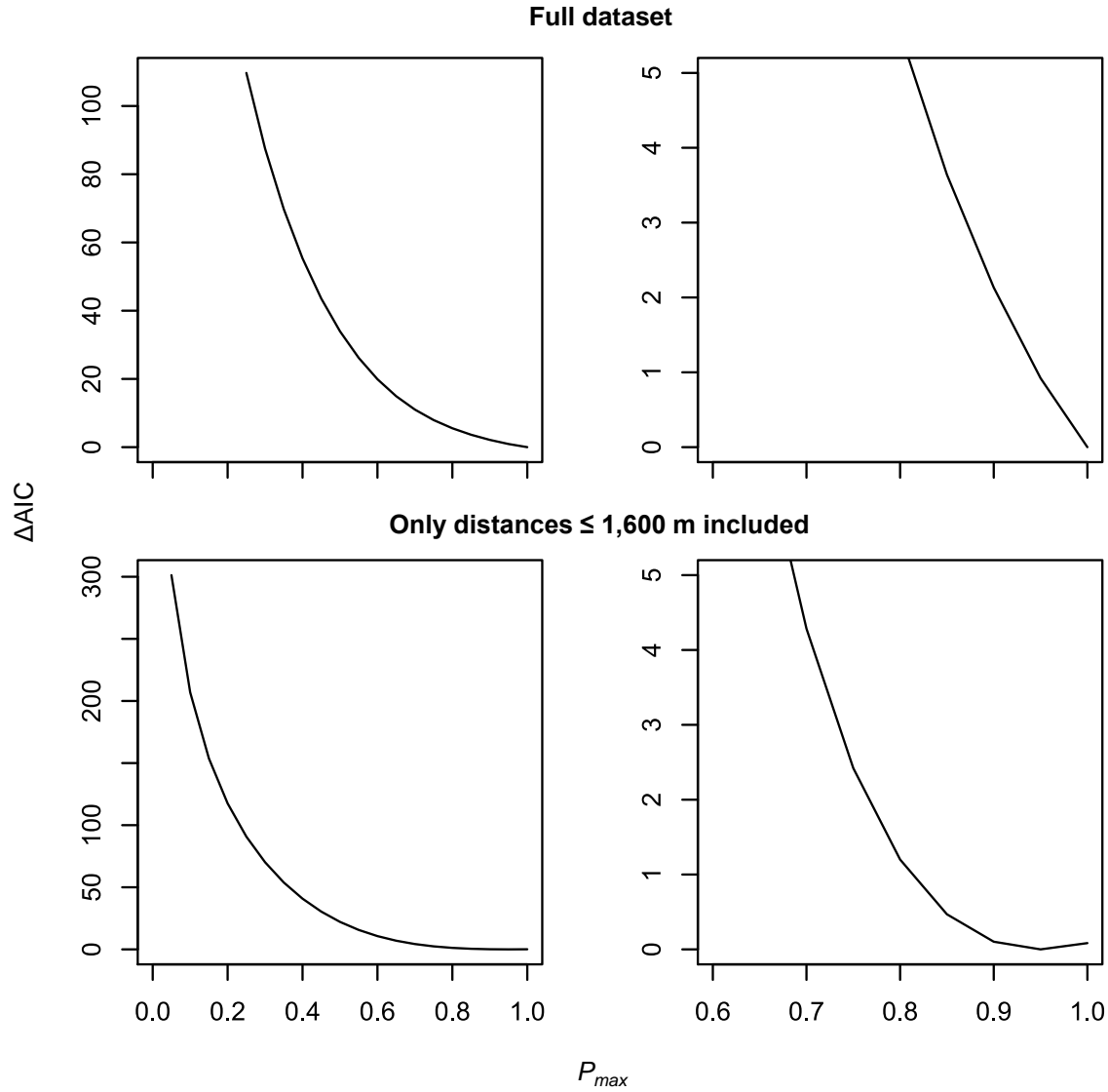
Figure S-3. AIC versus theoretical maximum eDNA proportion at banks downstream from fish ( P_{max} ) for the full and reduced dataset. The reduced dataset excludes distances > 1600 m, which were not sampled for all streams. Even lateral eDNA dispersion across a stream (i.e. across one midstream and both bankside samples) would result in an optimum P_{max} value of 0.67.
