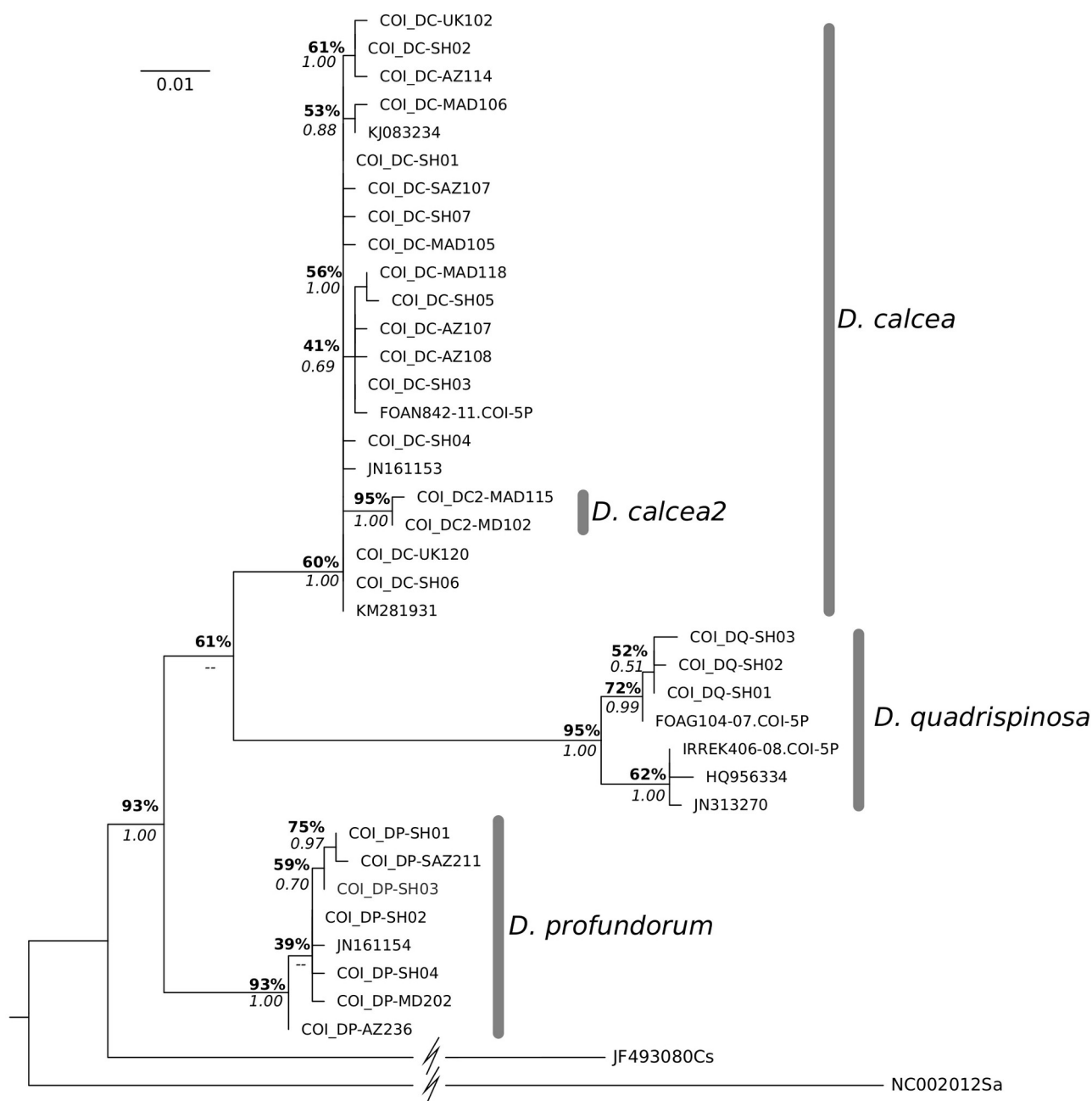
Supplementary Figure S1. Bayesian phylogenetic tree of Deania species obtained using COI sequences. Values at branches represent Bayesian posterior probabilities and bootstrap values obtained for the Maximum Likelihood tree. Nodes where Bayesian posterior probability was under 0.50 are not reported.
