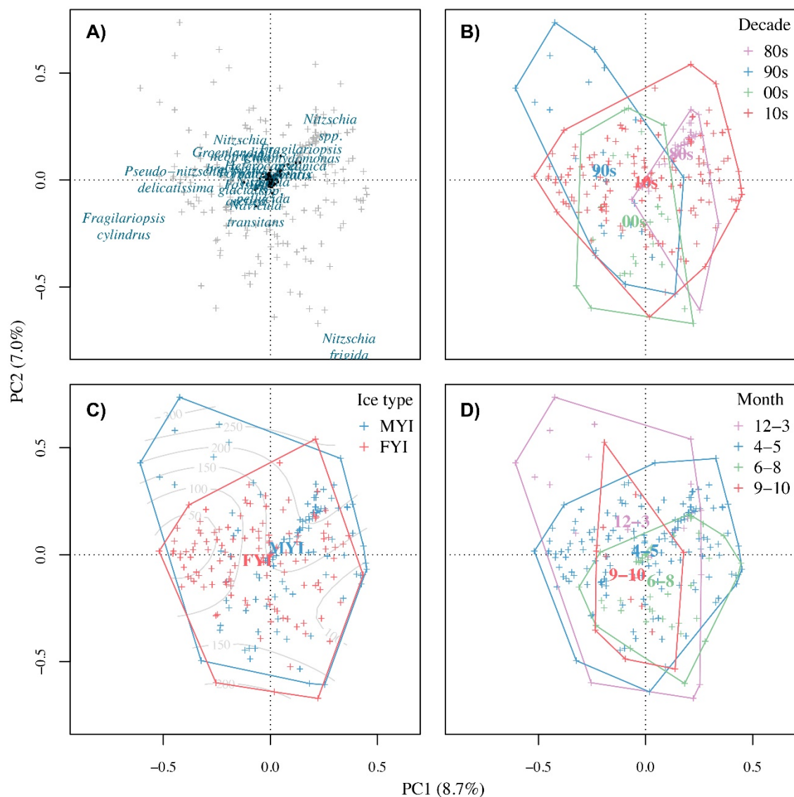
Figure S2. Principal component analysis conditioned with a dataset and sampled ice core length. (A) Overview of species (black dots and blue text) relation to ice cores (crosses). Ice cores related to decade (B), ice type (C), and month (D). Contours in C refer to ice thickness in cm.
