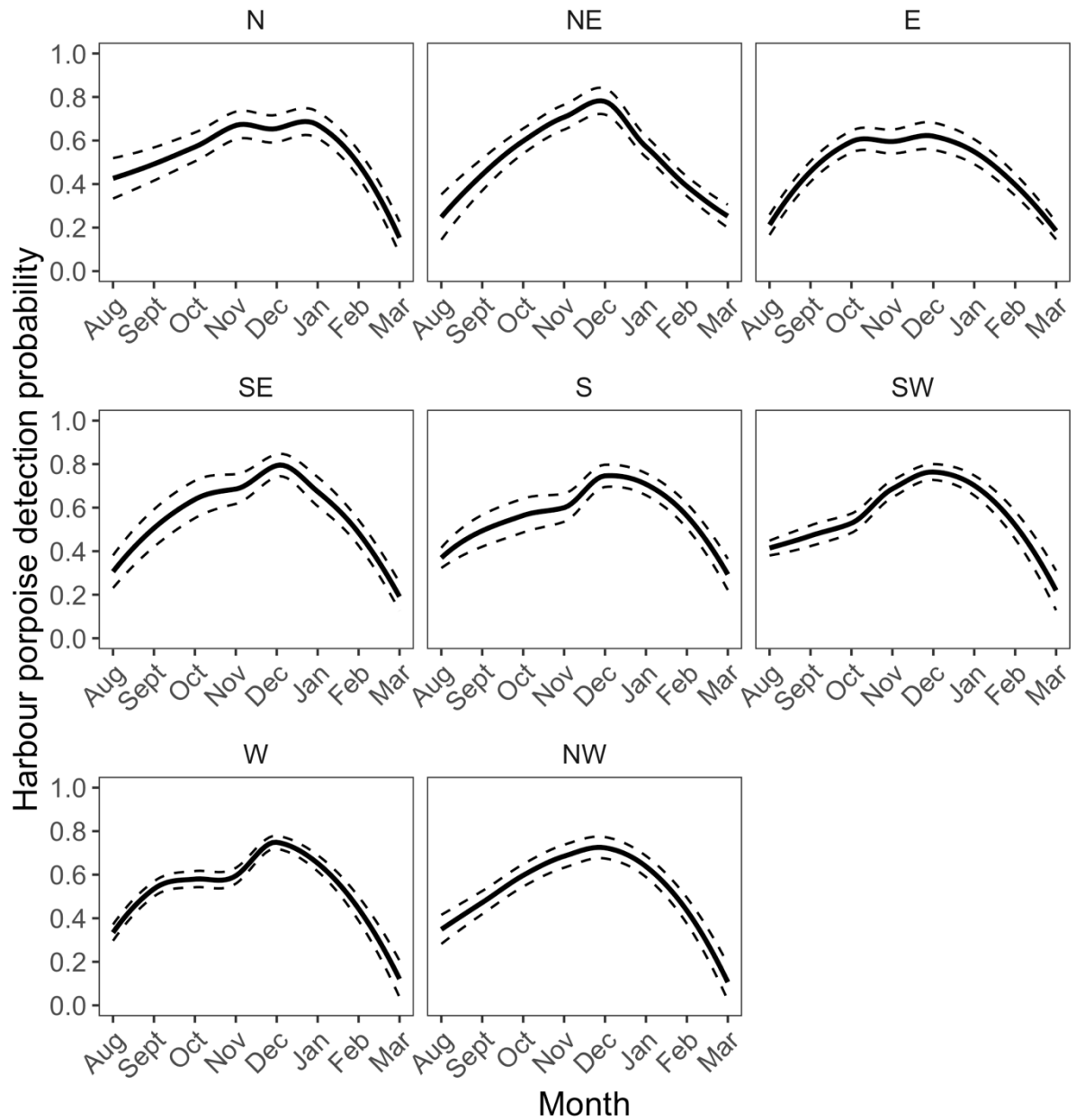
Figure S5. Effect of wind direction. Temporal variation of the probability of detecting harbour porpoises at the near C-POD for each wind direction. Solid lines denote predictions from top ranked models presented in Table 1. Standard errors are shown by the dashed lines.
