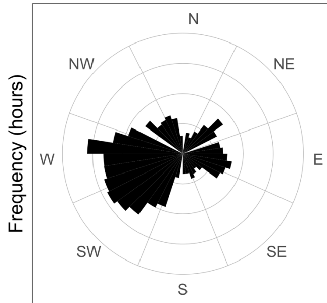
Figure S3. Frequency distribution of hourly averaged wind bearing over the study period. The y axis is represented by the concentric grey circles in 100 hr increments.
