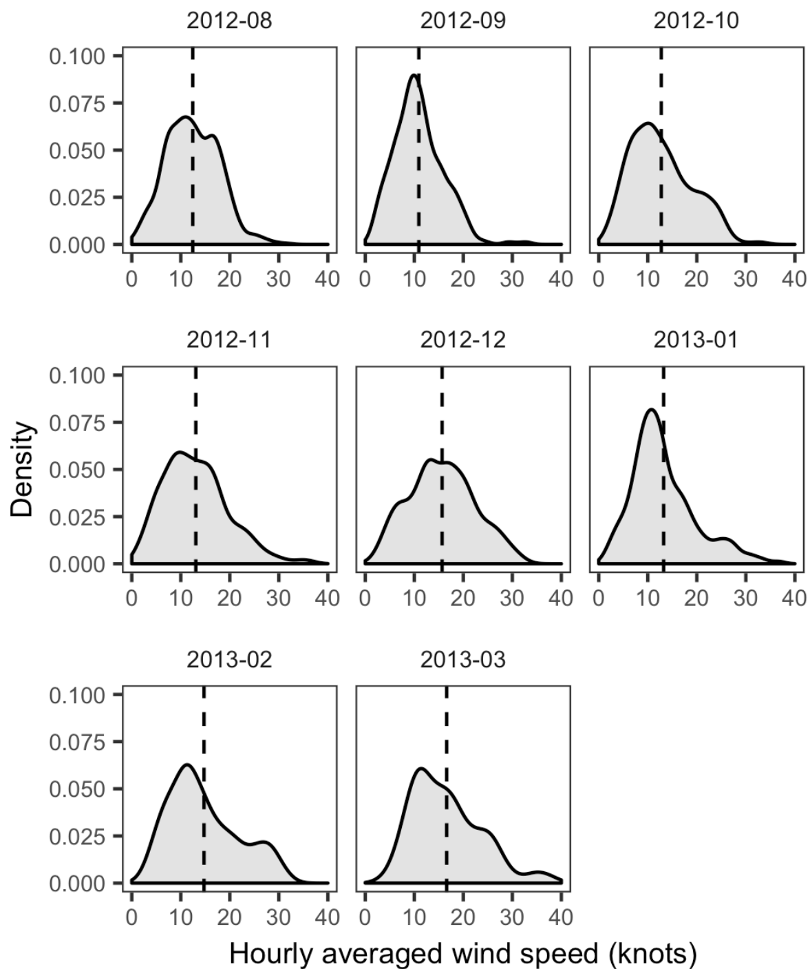
Figure S2. Monthly density plots of hourly averaged wind speed (knots) over the study period. The vertical dashed line represents the mean wind speed for each month.
