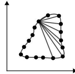
Fig. 26: Creating mass
