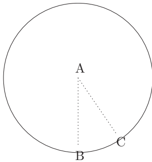
Fig. 44: Two points on the circumference
