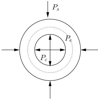
Fig. 20: Mass emergence
