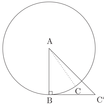
Fig. 45: The arc side
