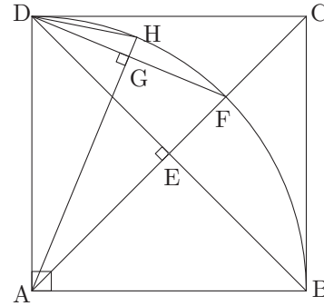
Fig. 49: The quarter slice of Fig. 48
