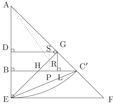
Fig. 47: A part of Fig. 46
