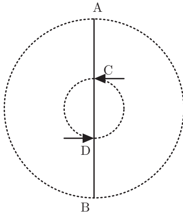
Fig. 43: An object which is about to go at light speed
