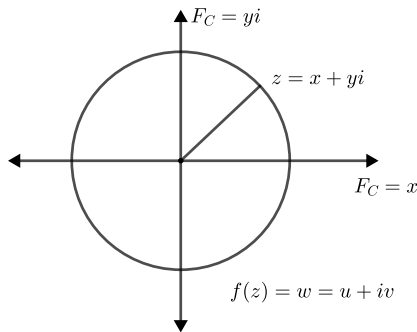
Fig. 29: Complex plane
