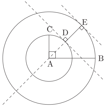
Fig. 50: The area scanned
