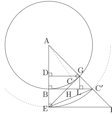
Fig. 46: The second radius
