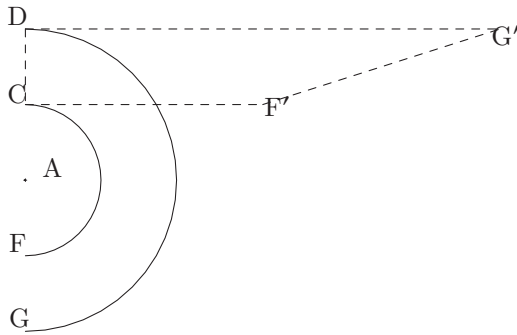
Fig. 51: The area of the circle in the kind of triangle
