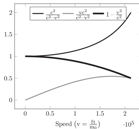
Fig. 33: Mass, length contraction and speed changing graphic from m = m_0 to m = 2m_0 , and L = L_0 to L = L_0/2
