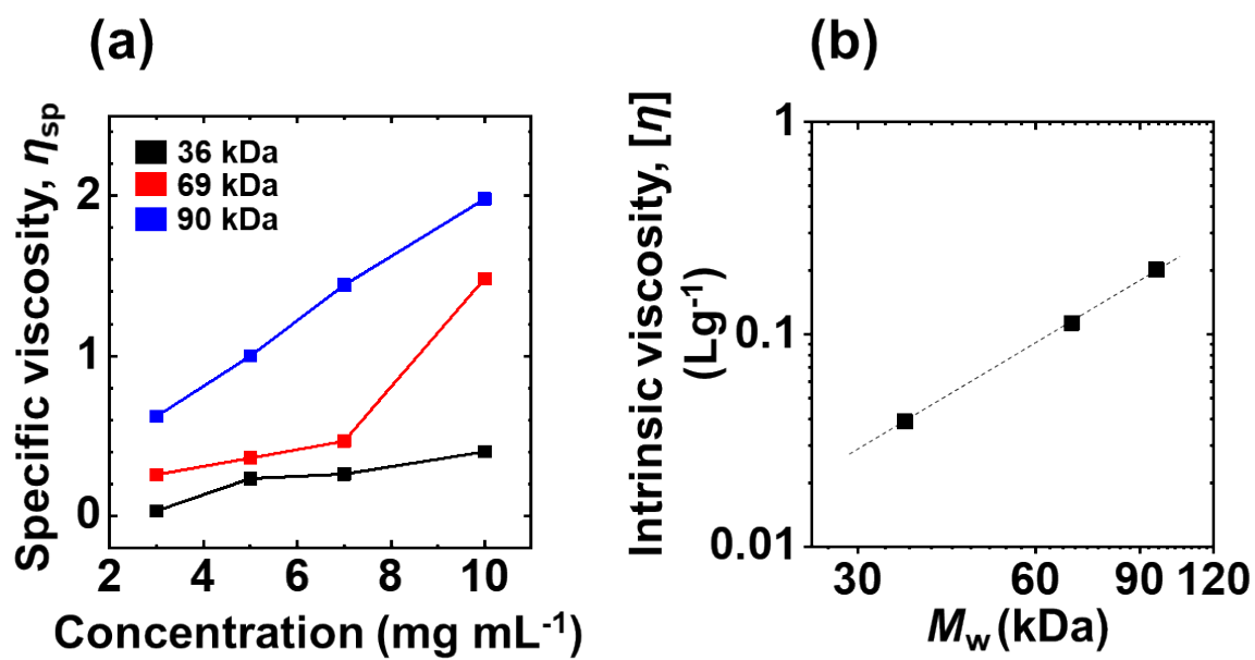
Figure S1. (a) Specific viscosities \eta_{sp} of the different M_w P3HT solutions as a function of the solution concentration. (b) Intrinsic viscosities [\eta] estimated from Figure S1a.
