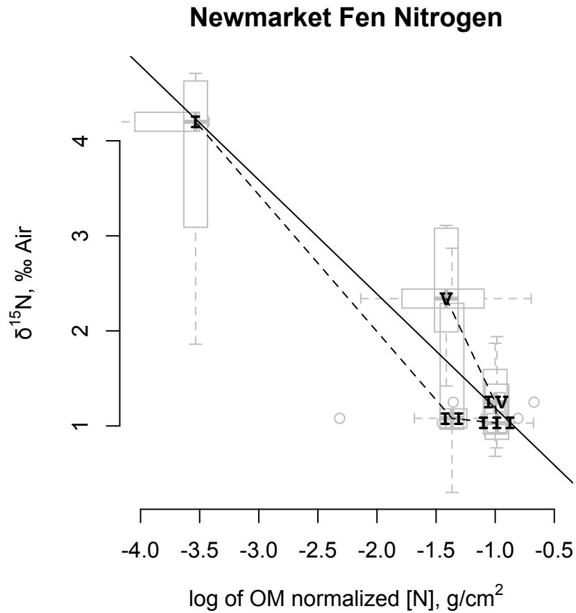
Figure S2: Two-direction box-and-whisker plots for Newmarket Fen nitrogen concentration and isotope data. Data are binned by macrofossil zone (roman numerals). Thick gray lines indicate median, box shoulders indicate interquartile range, and whiskers indicate 1.5 standard deviations. Solid black line is a least-squares fit, and dashed line connects medians in stratigraphic order.
