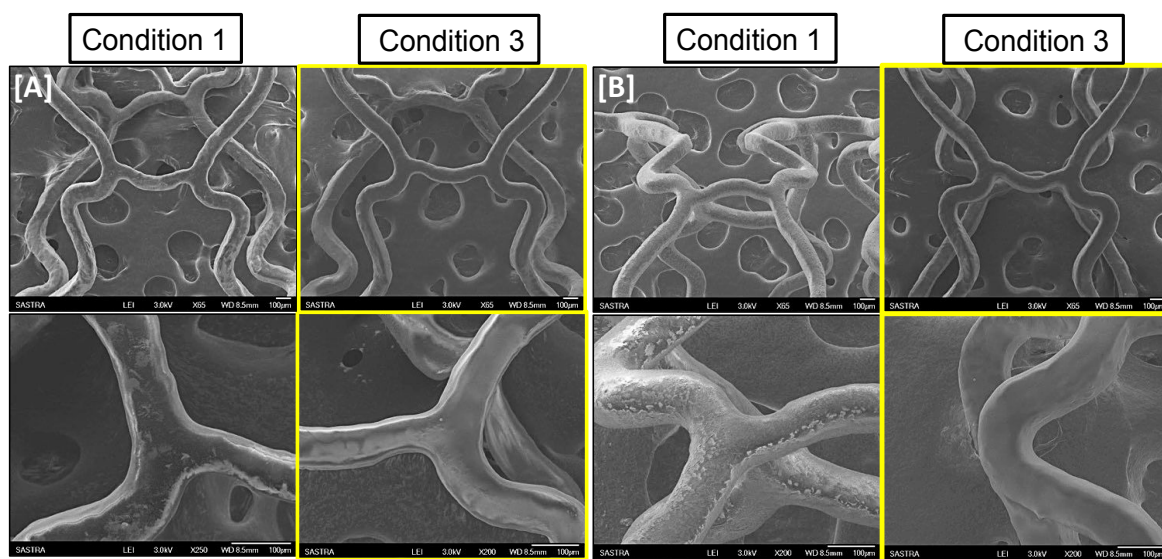
Figure S1. FE-SEM images of [A] atorvastatin and [B] fenofibrate loaded PLCL coated stents at two different sets of coating conditions.
