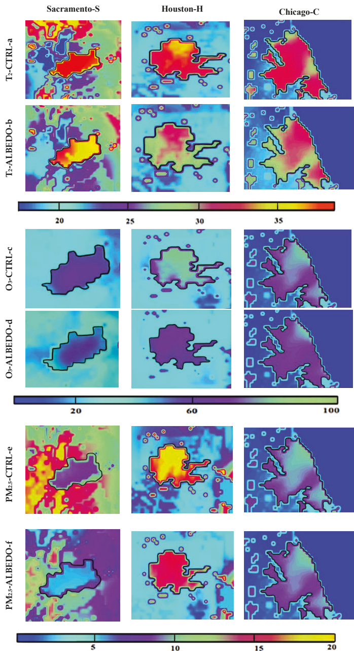
Figure 8. The maximum 2-m air temperature ( ^{\circ}C ), PM_{2.5} ( \mu g/m^3 ) and O_3 (ppb) concentrations in CTRL and ALBEDO scenarios across Sacramento, Houston, and Chicago during the 2011 heat wave period.
