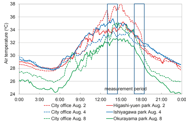
Figure 2. Measurement results of air temperature at the fixed measurement points.
