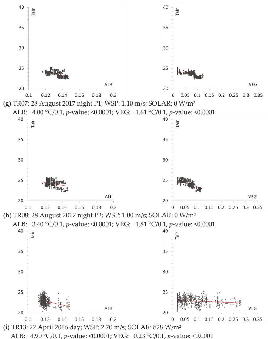
Figure 9. (a–i): Observed air temperature (from mobile transects) versus neighborhood-scale albedo and canopy cover in the downtown area. Vertical axis ( T_{\text{air}} ) is air temperature (°C); horizontal axis is albedo (ALB) or canopy cover (VEG), unitless.
