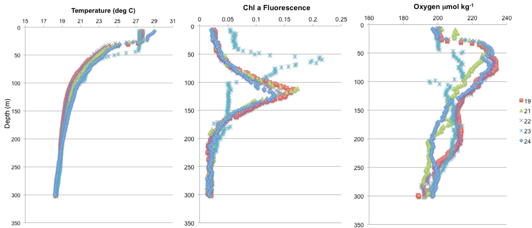
Figure S1. Temperature, chlorophyll a fluorescence, and oxygen profiles collected during the study in 19-24 August, 2014. The profiles were collected immediately before the first net tow at the station (see Table 1). The CTD was out of order on August 20 th .
