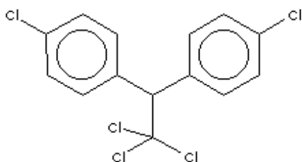
Scheme 1. Molecular structure of dichlorodiphenyltrichloroethane (DDT) ( C_{14}H_9Cl_5 ).
