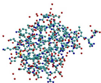
All atom representation
