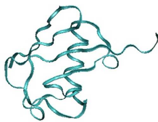
Ribbon representation
