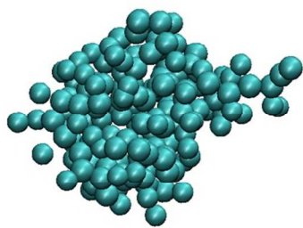
Coarse grained representation
