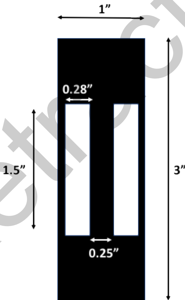
Figure S1. Mask for screen-printing of electrodes.
