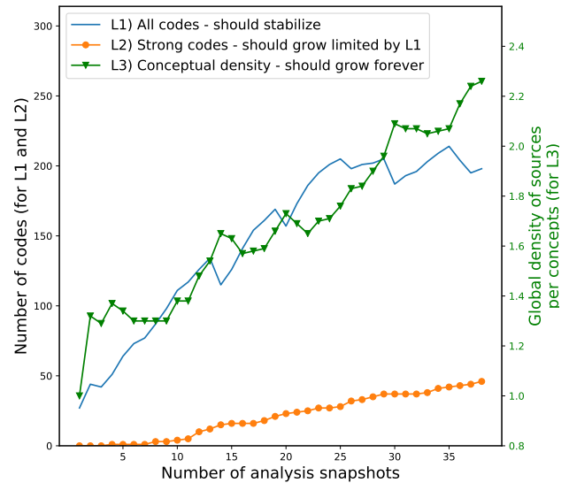
Fig. 2. Metrics of theoretical saturation for the 6C analysis
