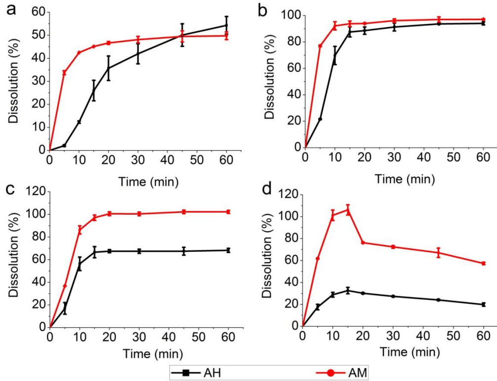
Figure S1. Sa to Sd are the dissolution profiles of AM and AH in dissolution medium at pH values of 1.0, 2.0, 5.0, 6.0 (data were expressed as mean \pm SD, n = 3 ).
