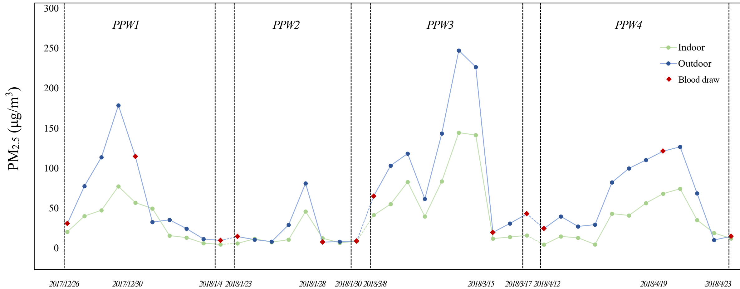
Figure S1 Time-varying outdoor and indoor PM 2.5 concentrations and the dates of blood draws over the study
