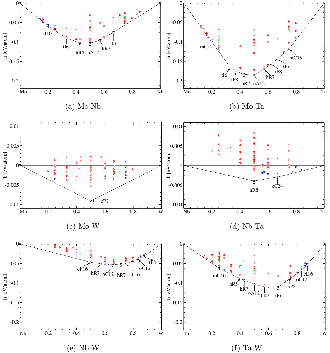
FIG. 1: First principles enthalpies of formation for binaries. Black squares denotes structures on the convex hull, blue squares denotes structures within 2 meV/atom of the convex hull, and red squares above 2 meV/atom. Filled green diamonds denote 16 atom BCC SQS (special quasirandom structures) [19]. The scales of Mo-W and Nb-Ta differ from the scales from the other four binaries.
