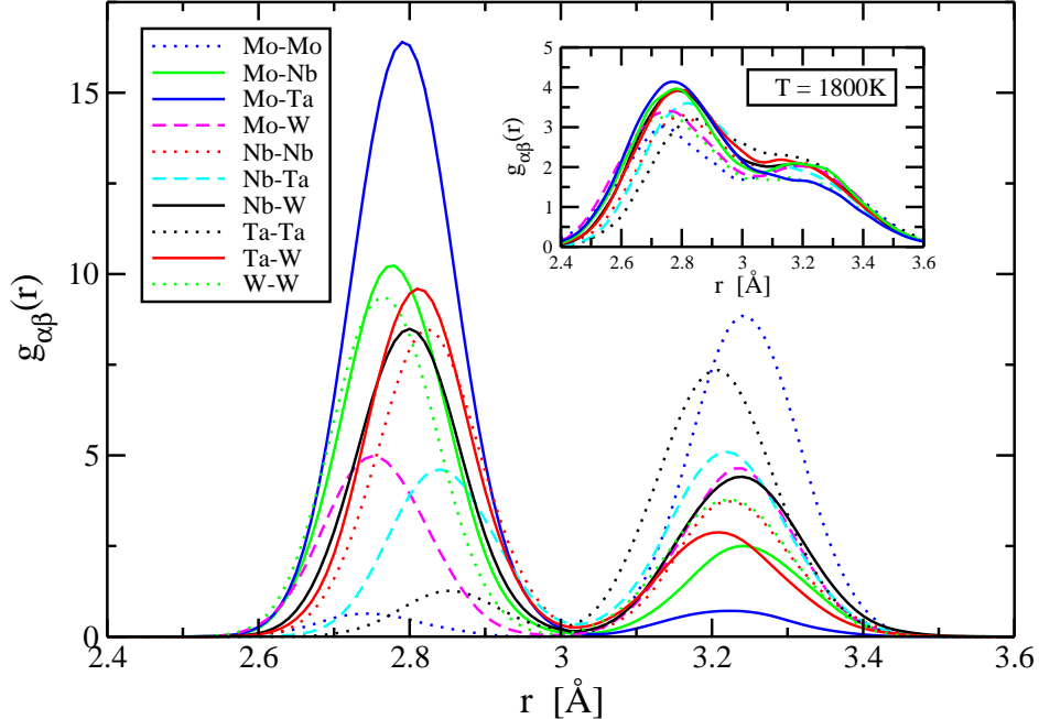
FIG. 2: Partial density functions obtained from MC/MD for the MoNbTaW BCC phase, showing first and second nearest neighbors. Solid lines denote PDFs between species from differing groups, dashed lines between differing species from the same group, and dotted lines between the same species. The main figure shows results for T=300\text{K} , and the inset for T=1800\text{K}
