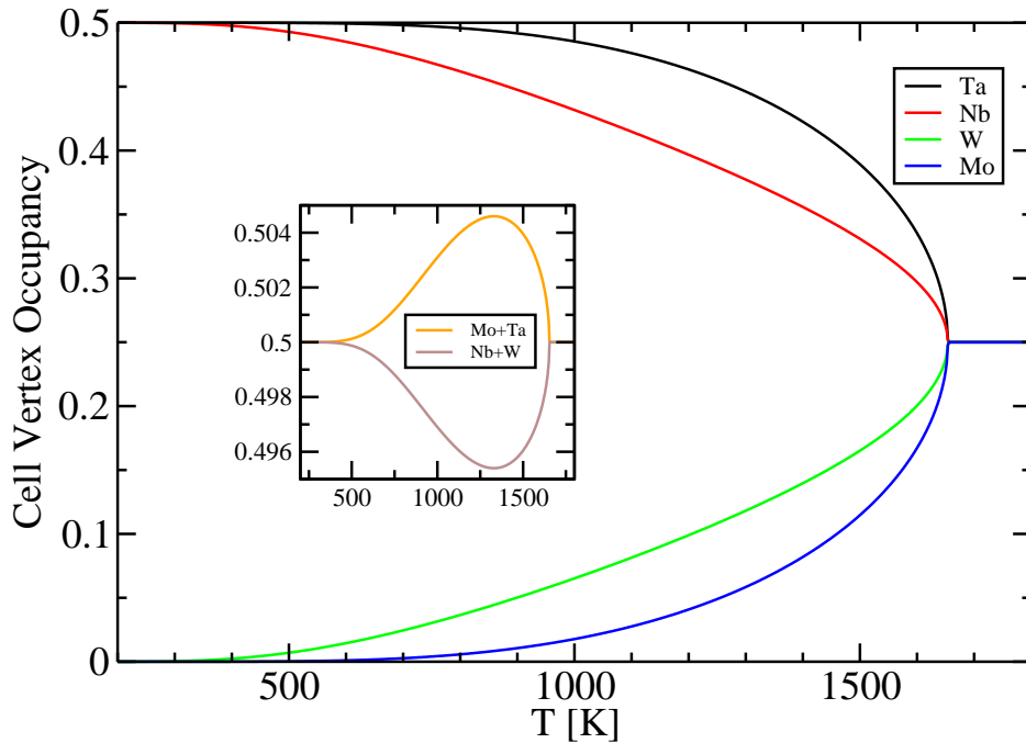
FIG. 3: The vertex sublattice occupancy as a function of temperature. See text for information on inset.
