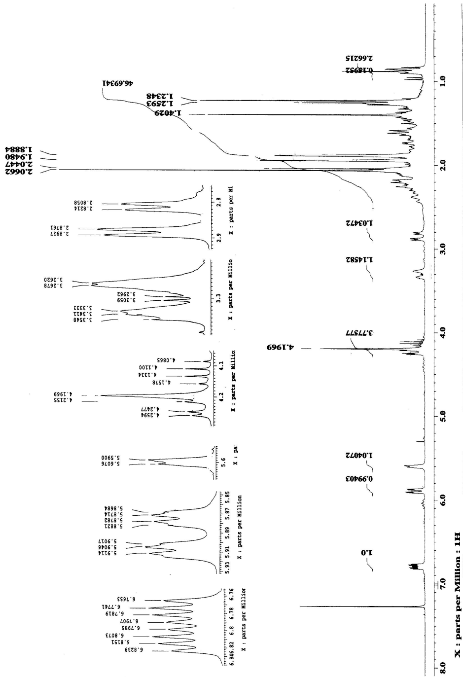
1 H NMR spectrum of physacoztotide E (9)
