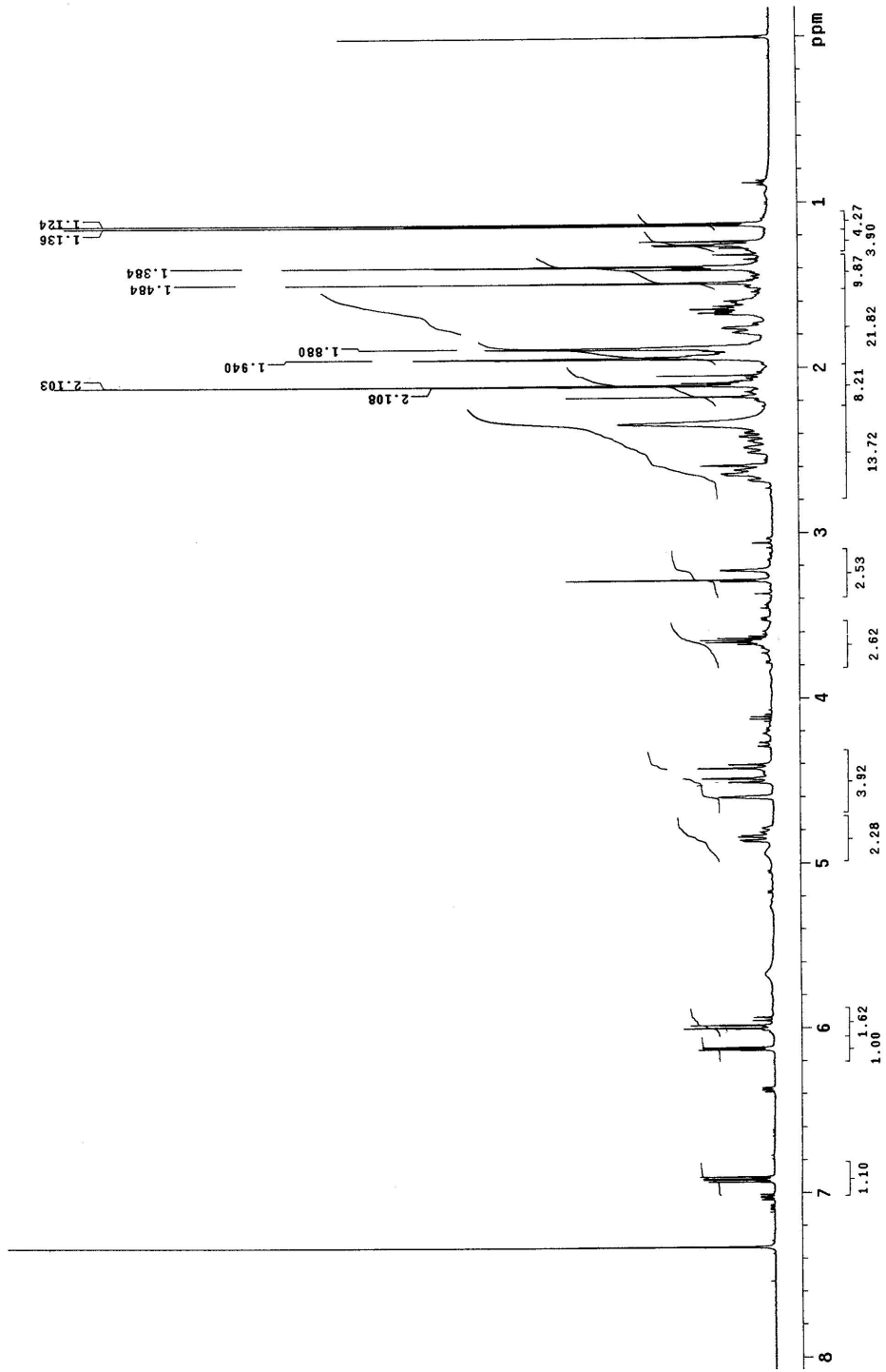
^1\text{H} NMR spectrum of physacoztolide D (8)
