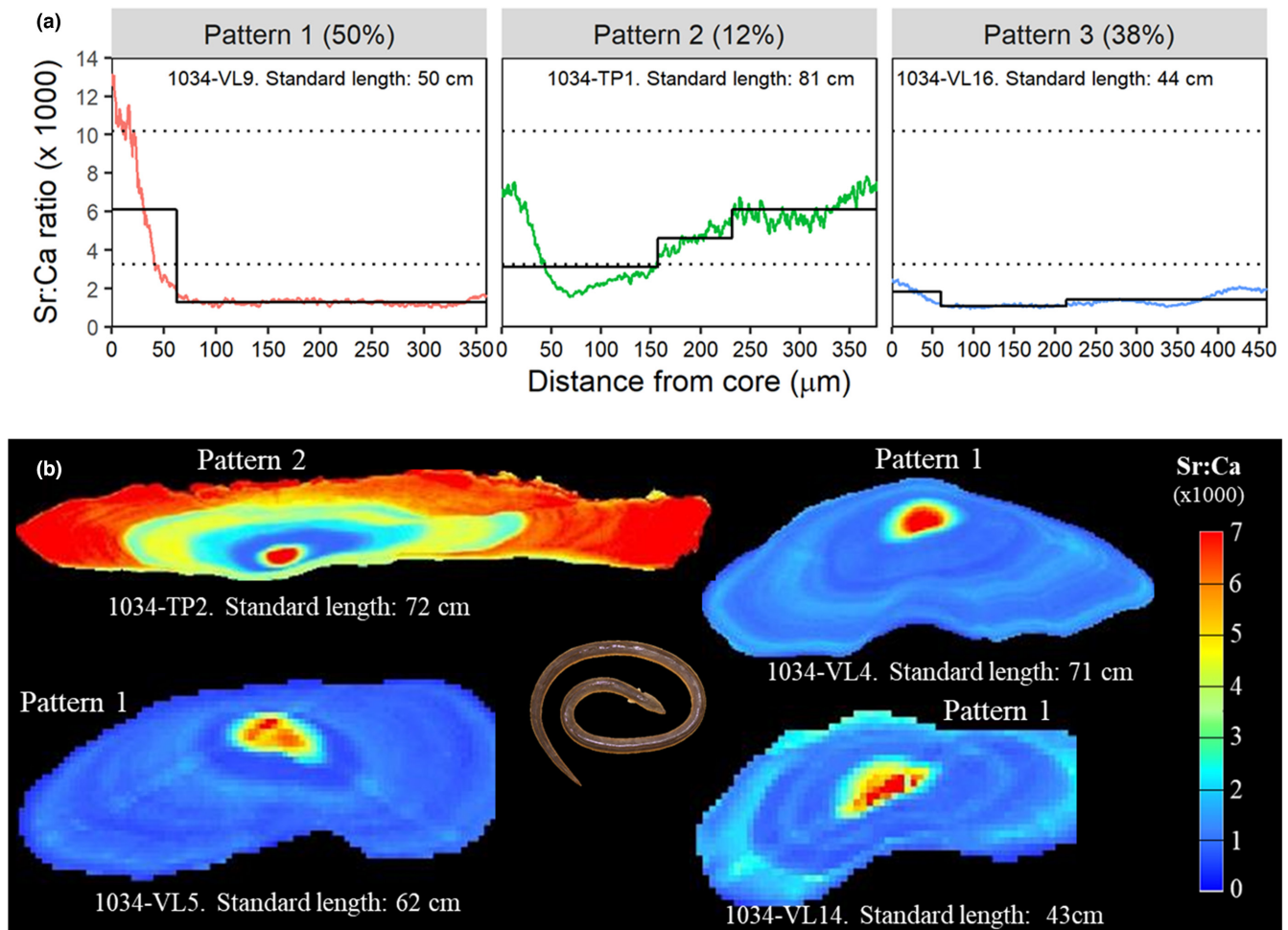
FIGURE 6 Variations of Sr:Ca ratios from core to edge of otoliths of Pisodonophis boro . (a) Black solid lines indicate Sr:Ca ratios that are chemically different between two adjacent zones; dashed horizontal lines are environmental thresholds: freshwater residence if y < 3.25 ; brackish water residence if 3.25 \leq y < 10.17 ; and marine water residence if y > 10.17 . Black lines indicate Sr:Ca ratios that are chemically different between two adjacent zones (identified by regime shift analysis). (b) Two-dimensional Sr:Ca ratio maps (only two patterns are showed; all transverse sections, except the 1034-TP2: frontal section). See Appendix S3 for individual plots of Sr:Ca ratios and Ba:Ca ratios. Specimen codes and total length are indicated
