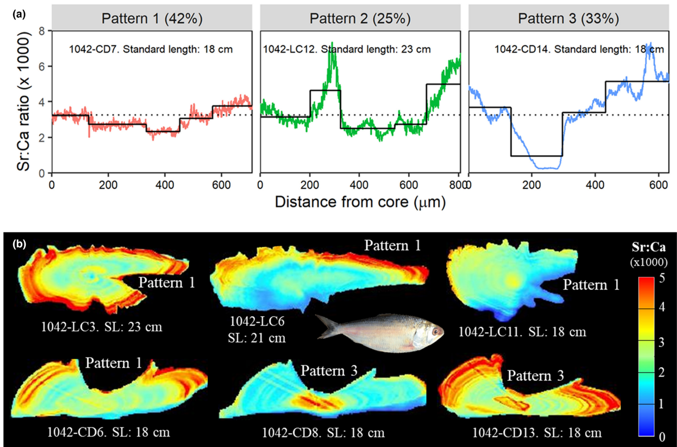
FIGURE 7 Variations of Sr:Ca ratios from core to edge of otoliths of Hilsa keele . (a) Black solid lines indicate Sr:Ca ratios that are chemically different between two adjacent zones; dashed horizontal lines are environmental thresholds: freshwater residence if y < 3.25 ; brackish water residence if 3.25 \leq y < 10.17 ; and marine water residence if y > 10.17 . Black lines indicate Sr:Ca ratios that are chemically different between two adjacent zones (identified by regime shift analysis). (b) Two-dimensional Sr:Ca ratio maps (only two patterns are showed; the top row are sagittal and the bottom row are transverse sections). See Appendix S3 for individual plots of Sr:Ca ratios and Ba:Ca ratios. Specimen codes and fork length are indicated
