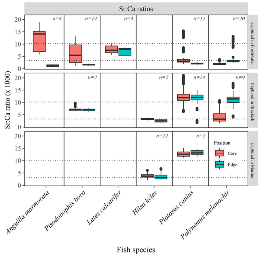
FIGURE 3 Box plots showing variations of Sr:Ca ratios at the core (birth: in orange) and edge (capture: in green) of otoliths of Mekong fishes at different capture environments. Box plots show minimum, maximum, and median values, outliers (data points lay outside the whiskers at 1.5 times the interquartile range above the upper quartile and below the lower quartile), and interquartile range in the data set. “ n ” indicates sample sizes. Dashed horizontal lines are environmental thresholds (freshwater residence if y < 3.25 ; brackish water residence if 3.25 \leq y < 10.17 ; and marine water residence if y > 10.17 ). See Appendix S2 for Ba:Ca ratios
