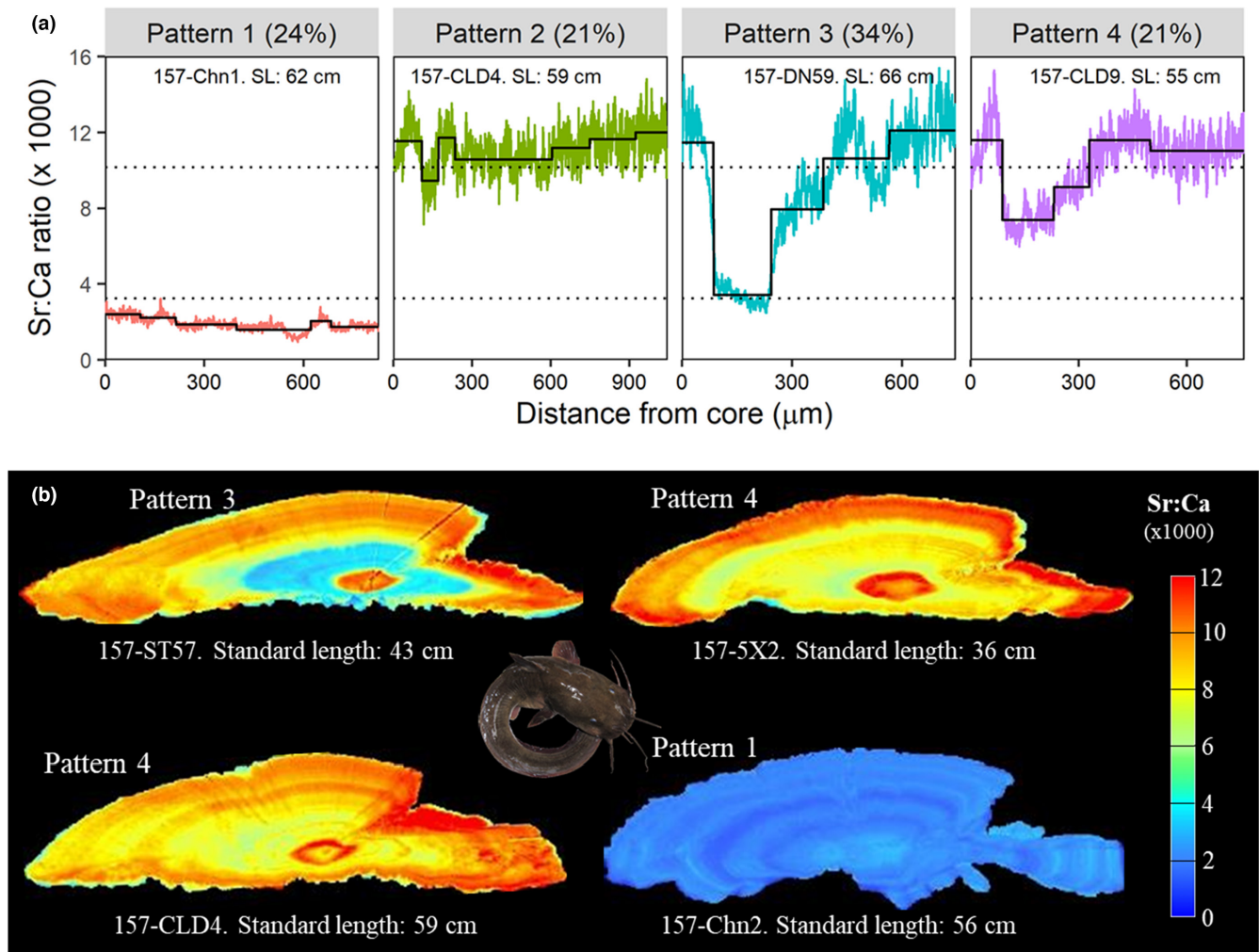
FIGURE 8 Variations of Sr:Ca ratios from core to edge of otoliths of Plotosus canius . (a) Black solid lines indicate Sr:Ca ratios that are chemically different between two adjacent zones; dashed horizontal lines are environmental thresholds: freshwater residence if y < 3.25 ; brackish water residence if 3.25 \leq y < 10.17 ; and marine water residence if y > 10.17 . Black lines indicate Sr:Ca ratios that are chemically different between two adjacent zones (identified by regime shift analysis). (b) Two-dimensional Sr:Ca ratio maps. See Appendix S3 for individual plots of Sr:Ca ratios and Ba:Ca ratios. Specimen codes and total length are indicated
