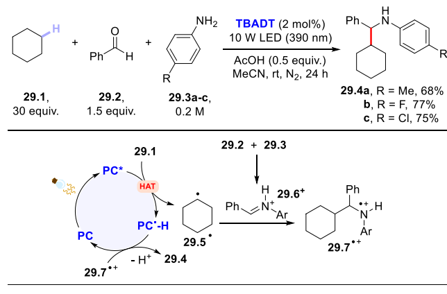
Scheme 29. Multicomponent Synthesis of Secondary Amines
