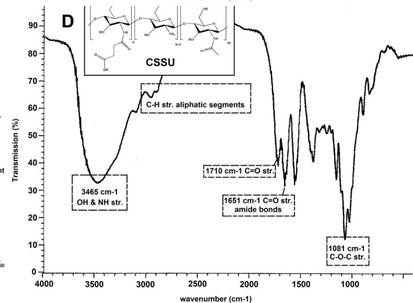
Figure S1: the FTIR spectra for CS (A), BPA-BOC (B), PNIPAAm (C), and CSSU (D)
