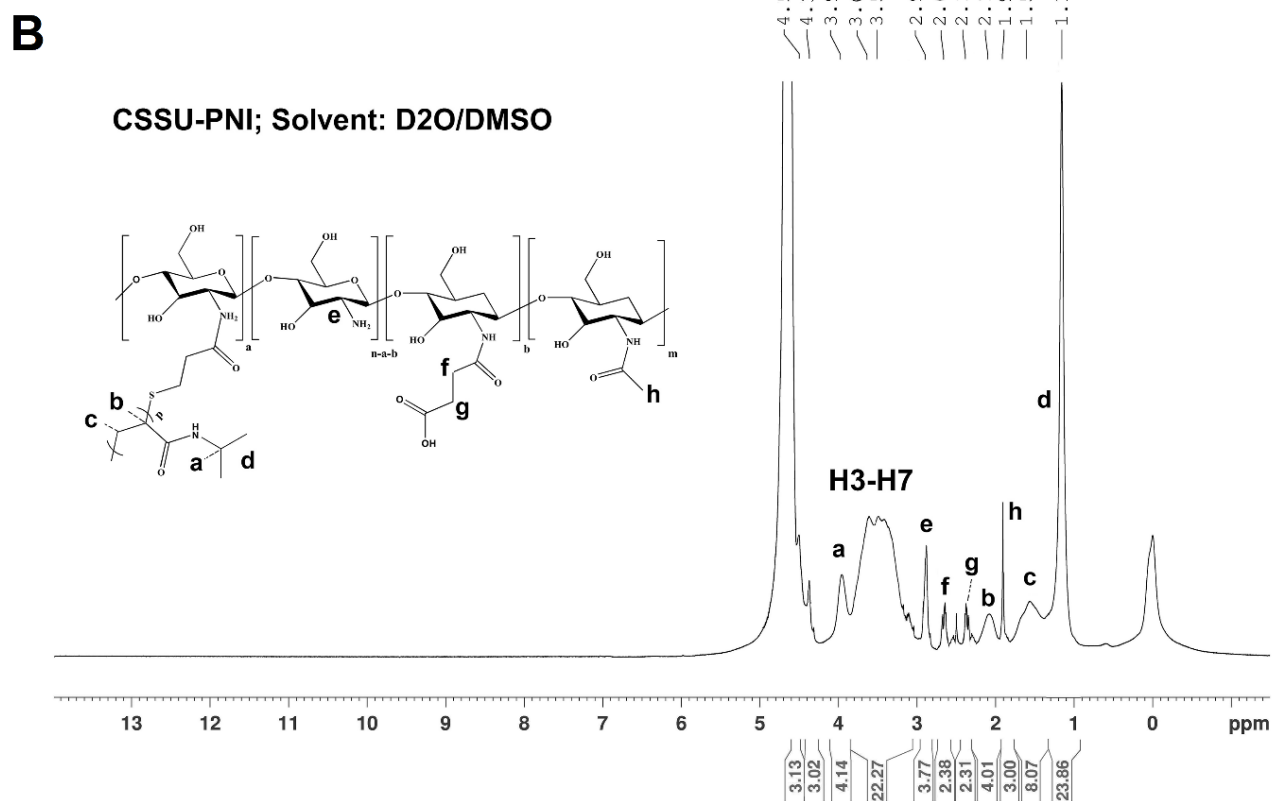
Figure S3: (A): the FTIR spectra for CSSU-PNI; (B): 1 H-NMR spectra of CSSU-PNI
