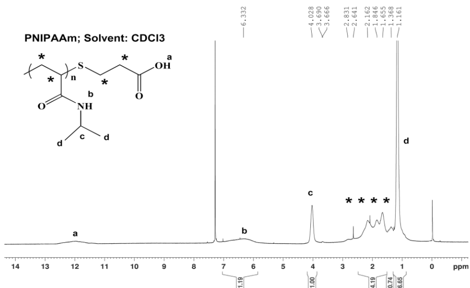
Figure S2: the 1 H NMR spectra for CS (A), BPA-BOC (B), PNIPAAm (C), and CSSU (D)
