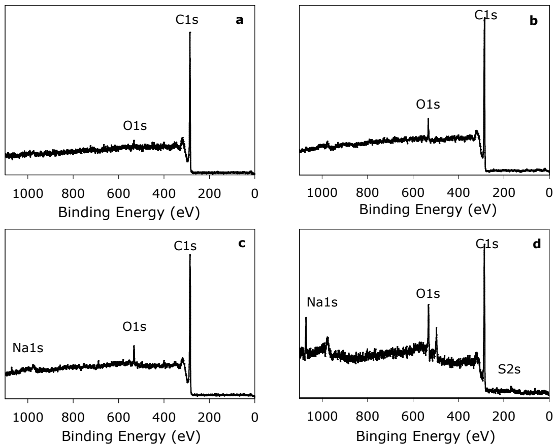
Figure SI-1. XPS survey analysis of (a) annealed nanodiamond 1 , (b) carboxylated nanodiamond 2 , (c) sodium salt of carboxylated nanodiamond 3 , (d) sodium salt of phenyl sulfonated nanodiamond 6 .
