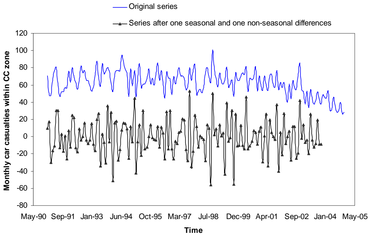
Figure 6: The differenced (seasonally and non-seasonally) monthly car casualty series for the congestion charging zone, from January 1991 to December 2004.
