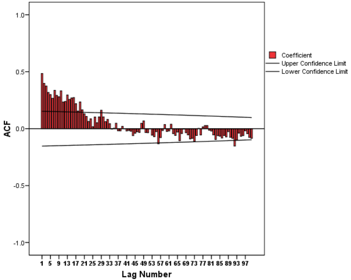
Figure 5: Sample ACF and 95% confidence limits for the monthly car casualties within the congestion charging zone (Jan 1991 to Dec 2004)
