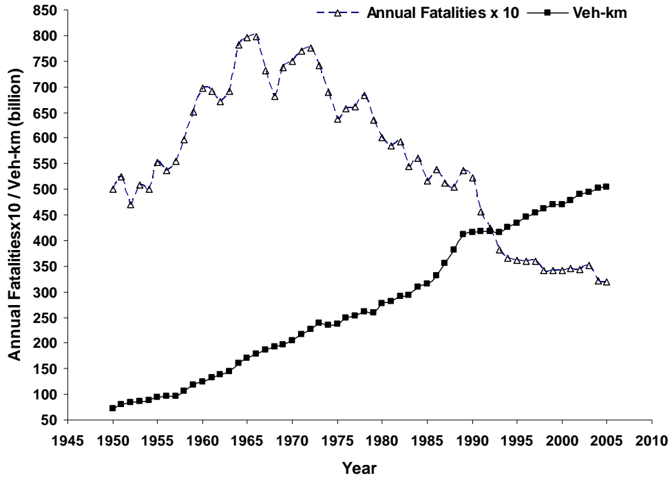
Figure 1: Annual road traffic fatalities and vehicle km travelled in GB
