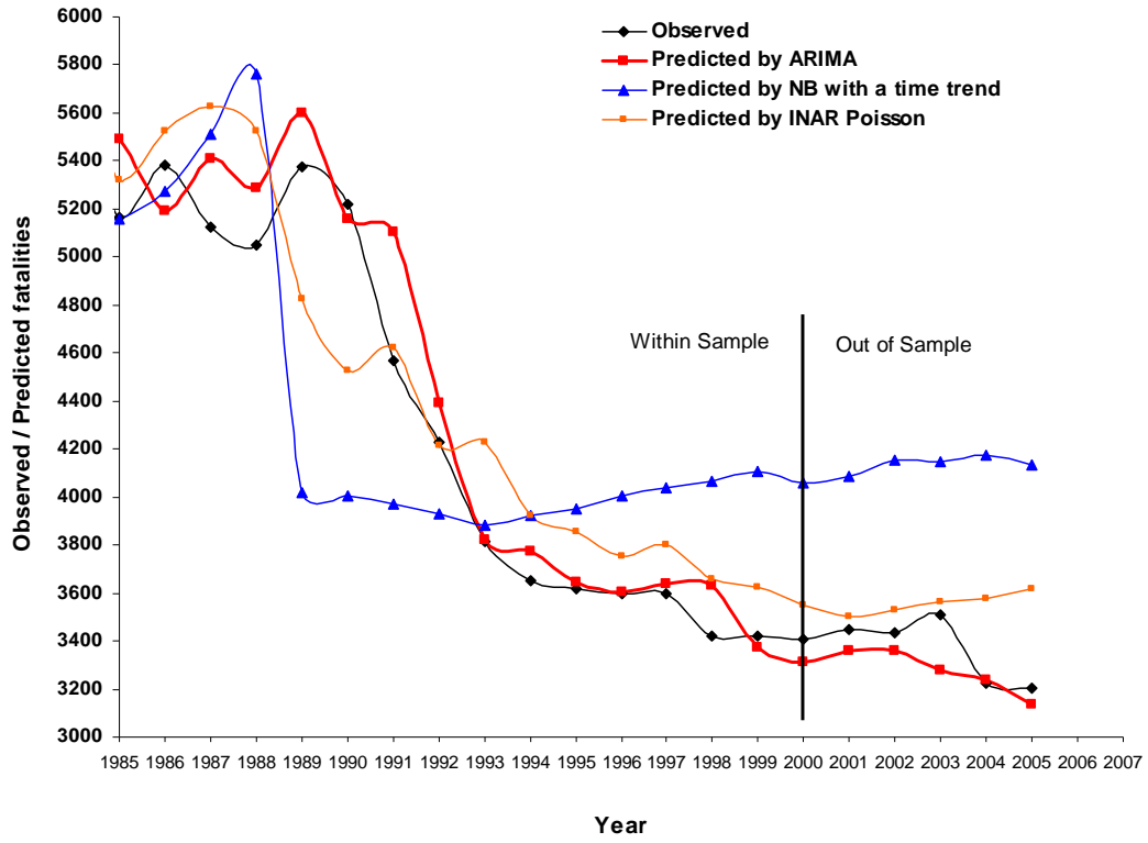
Figure 4: Observed vs Predicted values of fatalities
