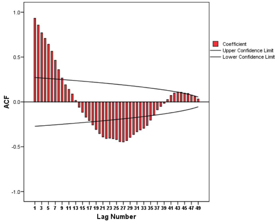
Figure 3: Sample ACF and 95% confidence limits for the yearly road fatalities in GB
