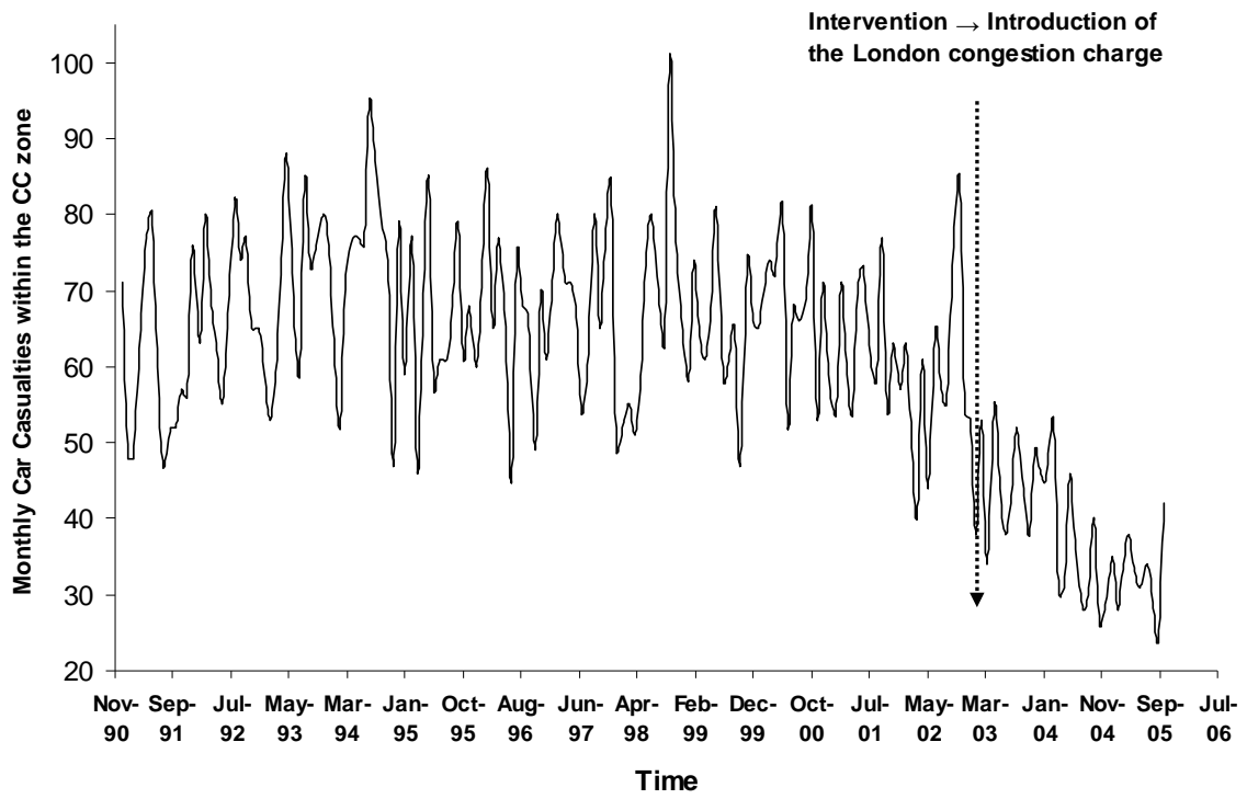
Figure 2: Monthly car casualties within the congestion charging zone (Jan 1991 to Oct 2005)
