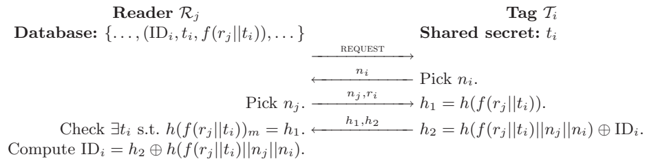
Fig. 4. The Auth2 protocol
