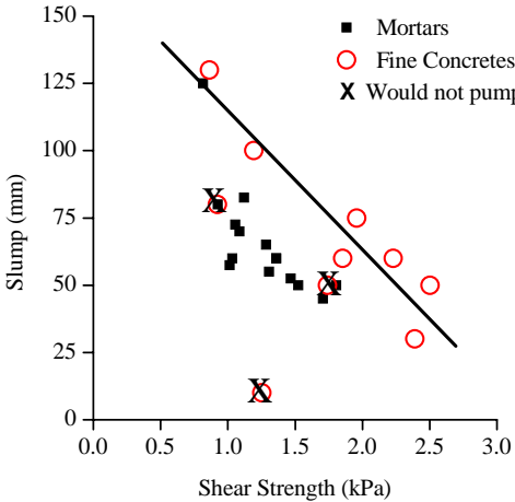
Figure 5(b). Relationship between slump and vane shear strength for fine concretes and mortars
