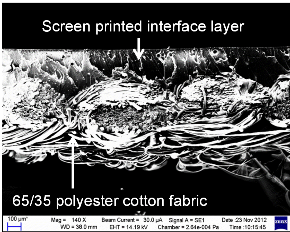
Figure 3. Cross sectional view SEM images of standard 65/35 polyester cotton fabric with interface layer
