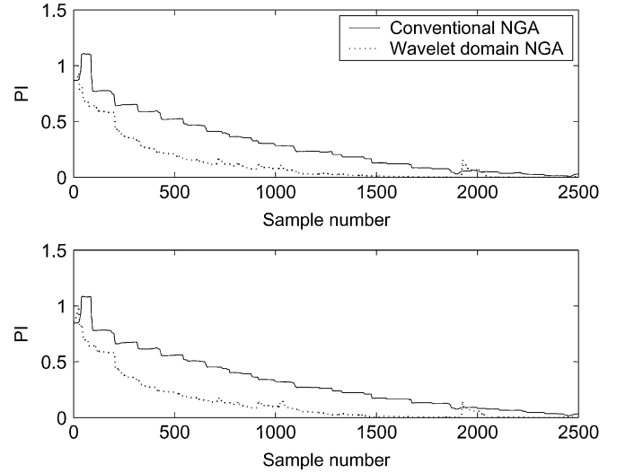
Fig. 10. Performance index obtained with NGA and NGA and wavelet transform, for the fetal and maternal ECG sources in Fig. 2, when zero mean Gaussian noise is present. The upper plots depict the PI when the SNR is 10 dB, while the lower plots correspond to a SNR of 5 dB.
