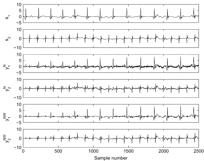
Fig. 12. Original MECCG and FECCG sources ( s_1 and s_2 ), and signals recovered by time domain NGA ( y_1^N and y_2^N ), and the wavelet domain method ( y_1^{NW} and y_2^{NW} ), when the SNR is 5 dB.
