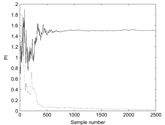
Fig. 14. Performance indices obtained for NGA (solid line), and wavelet domain NGA (dotted line), when the two original sources are sub-Gaussian and the nonlinearity is super-Gaussian.
