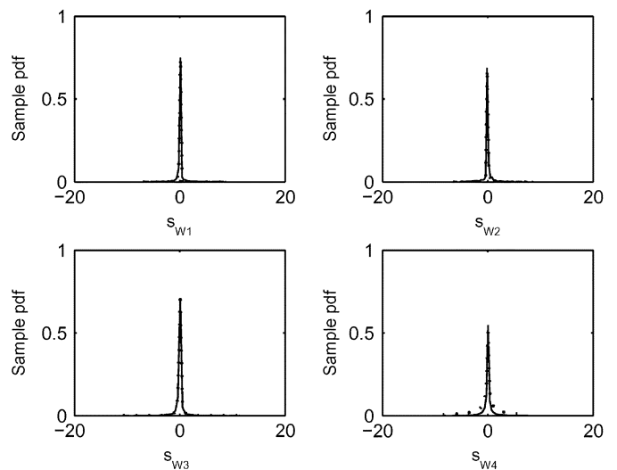
Fig. 3. Sample distributions (solid lines) and fitted Generalized Gaussian sample pdfs (dotted lines) for the wavelet coefficients of the sources in Fig. 2.
