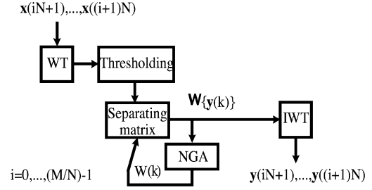
Fig. 7. Diagram of the NGA in the wavelet domain approach. The mixtures are divided into blocks of length N , so that the i th block is formed by samples \mathbf{x}(iN+1), \dots, \mathbf{x}((i+1)N) , where i = 0, \dots, (M/N)-1 . The wavelet transform of each block of data is then evaluated, and hard-thresholding is applied to the concatenated wavelet coefficients. NGA separates the transformed signals sequentially, giving a vector of estimated signals, whose inverse wavelet transform represents the corresponding block of recovered sources.
