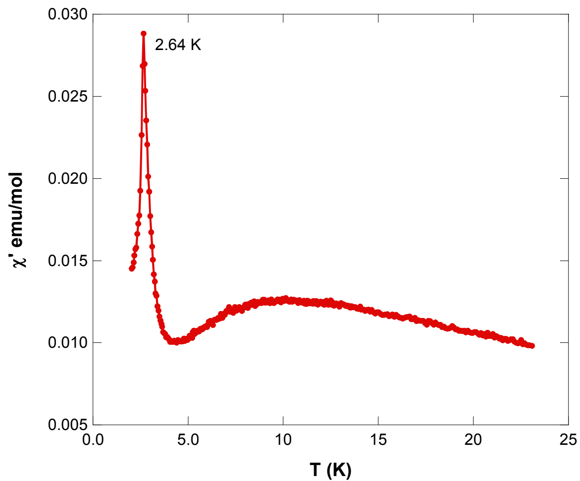
\chi''(T) plot for a polycrystalline sample of \text{CuF}_2(\text{H}_2\text{O})_2(\text{pyz}) . H_{\text{dc}} = 0 Oe, H_{\text{ac}} = 1 Oe, \omega = 125 Hz.
